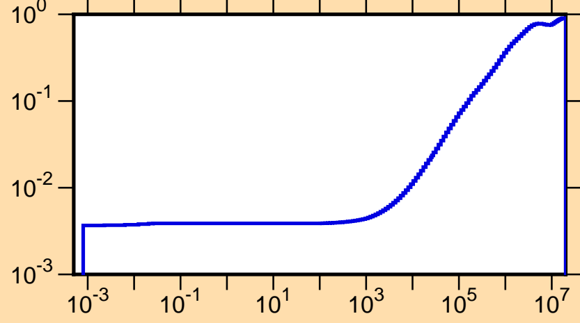
\mu vs. E for ^{184}\text{Au}(\text{mt251})
