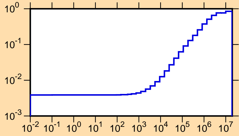
\mu vs. E for ^{184}\text{Au}(\text{mt251})
