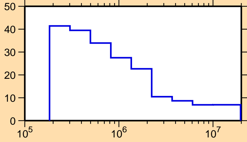
\Delta\sigma/\sigma vs. E for ^{184}\text{Au}(n,n\text{onel.})
