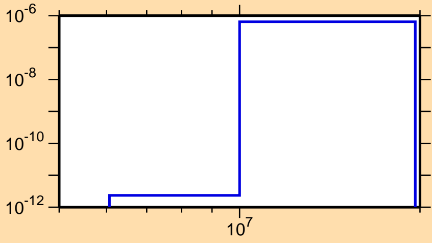
\sigma vs. E for ^{184}\text{Au}(\text{mt } 45)
