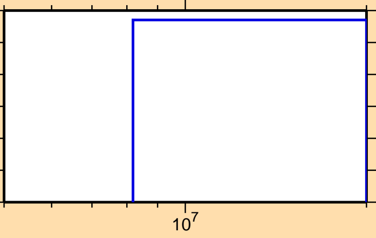
\sigma vs. E for ^{184}\text{Au}(n,\text{pd})
