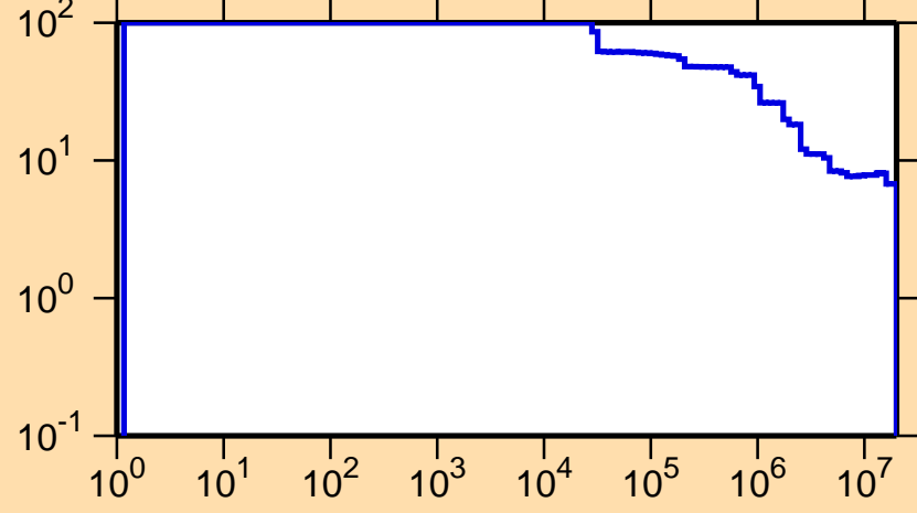
\Delta\sigma/\sigma vs. E for ^{184}\text{Au}(n,\text{nonel.})
