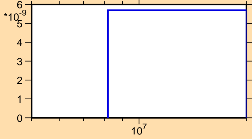
\sigma vs. E for ^{184}\text{Au}(n,\text{pd})
