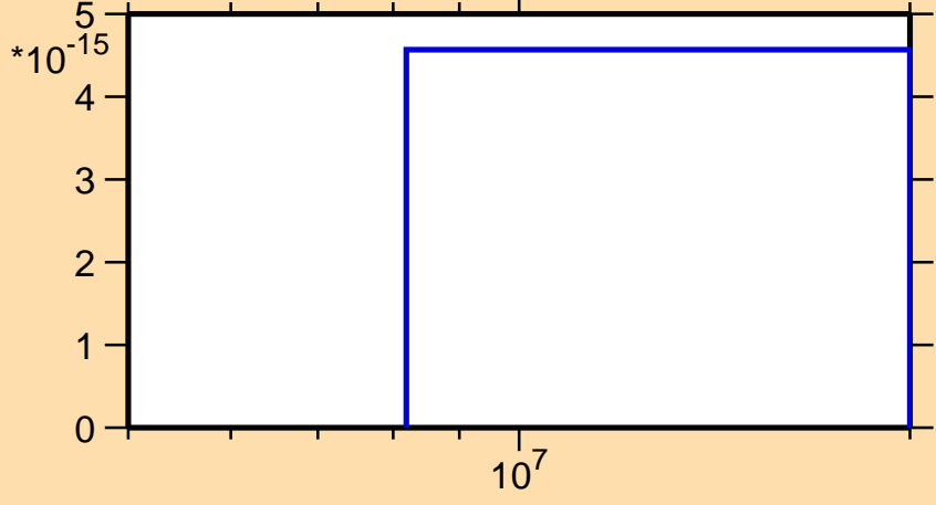
\sigma vs. E for ^{184}\text{Au}(n,3n\alpha)
