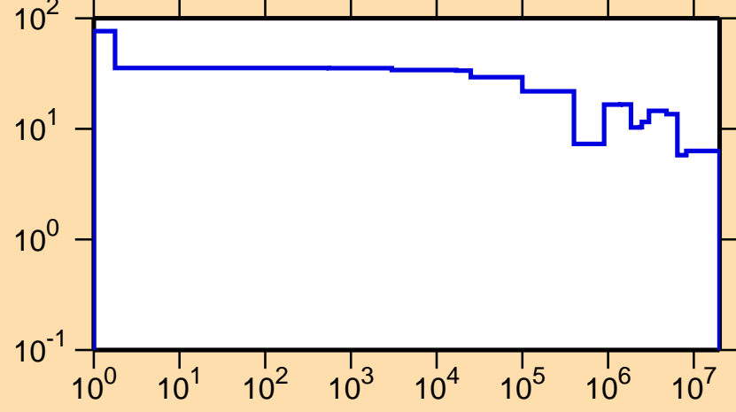
\Delta\sigma/\sigma vs. E for ^{184}\text{Au}(n,\text{el.})
