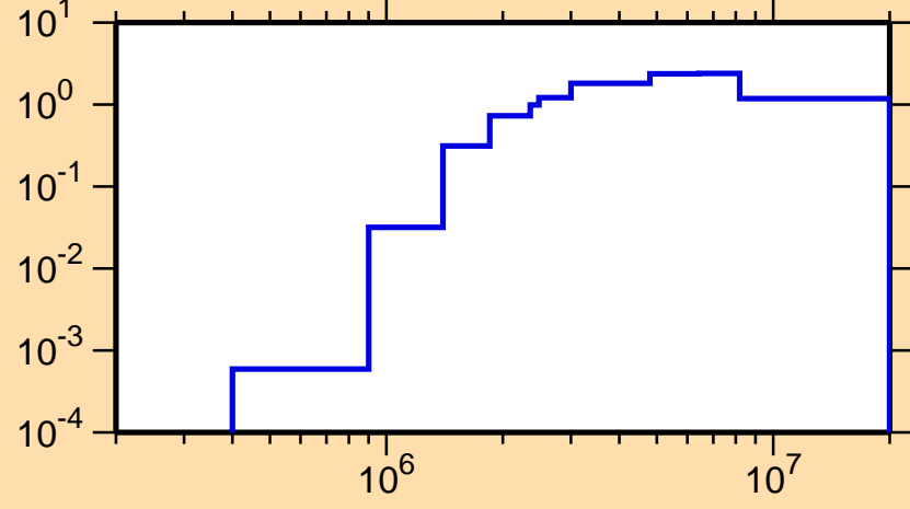
\sigma vs. E for ^{184}\text{Au}(n,n\text{cont.})
