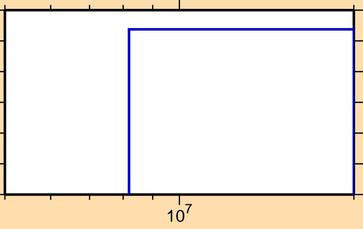
\sigma vs. E for ^{184}\text{Au}(\text{mt117})
