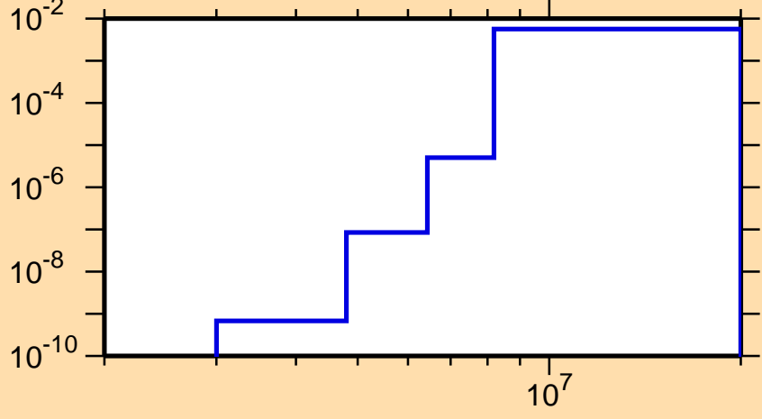
\sigma vs. E for ^{184}\text{Au}(n,d)
