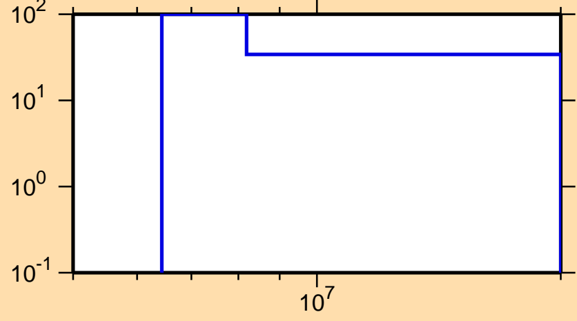
\Delta\sigma/\sigma vs. E for ^{184}\text{Au}(n,2n)
