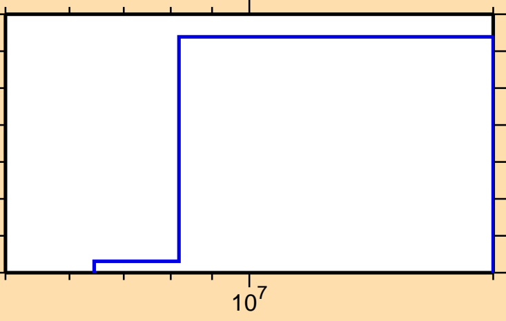
\sigma vs. E for ^{184}\text{Au}(n,\text{He3})
