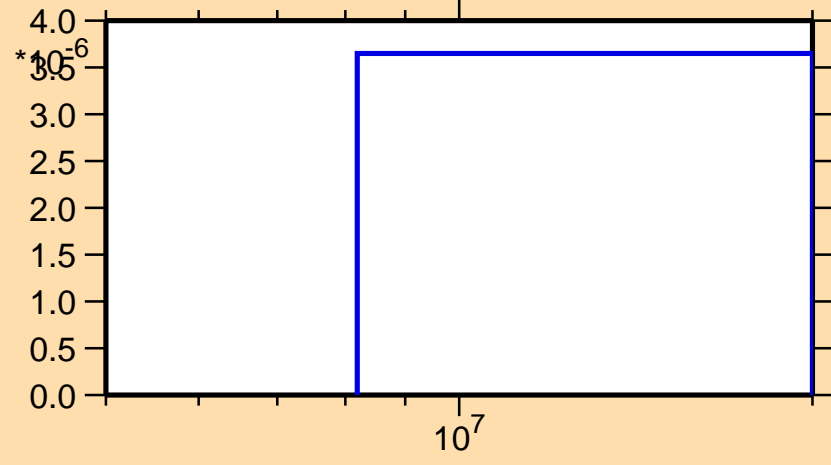
\sigma vs. E for ^{184}\text{Au}(n,\text{nd})
