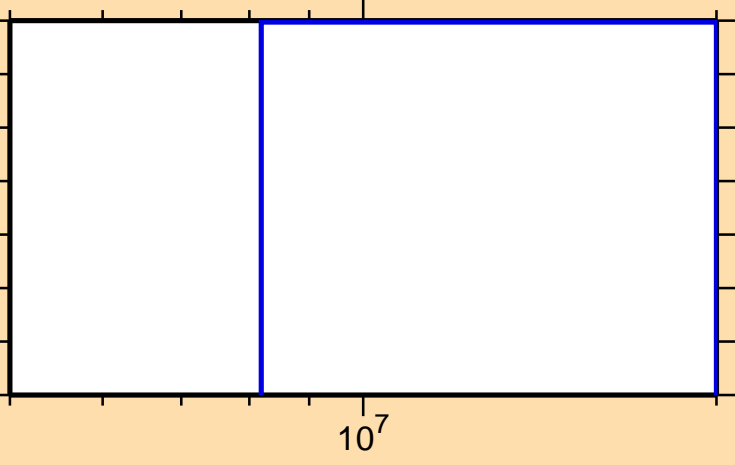
\sigma vs. E for ^{185}\text{Au}(n,\text{He3})
