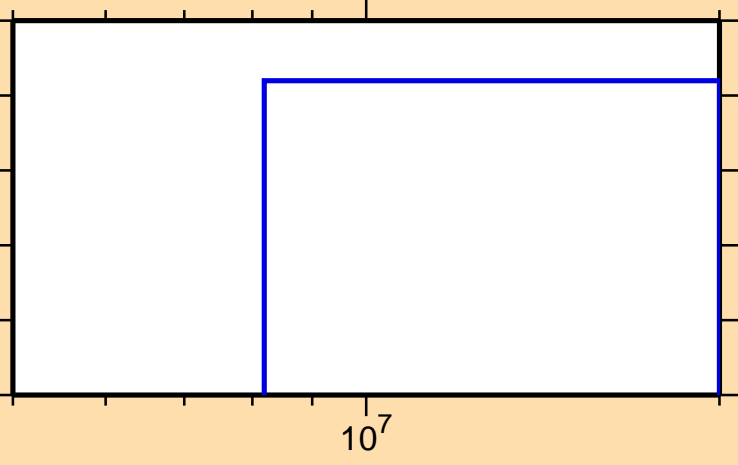
\sigma vs. E for ^{185}\text{Au}(n,\text{pd})
