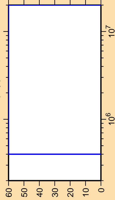
\Delta\sigma/\sigma vs. E for ^{185}\text{Au}(n,p)
