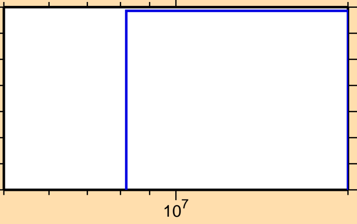
\sigma vs. E for ^{185}\text{Au}(n,2n\alpha)
