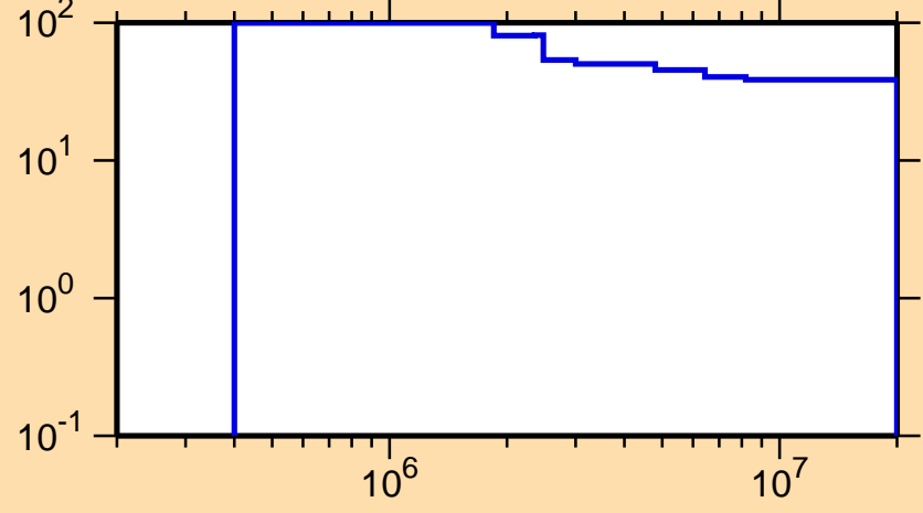
\Delta\sigma/\sigma vs. E for ^{185}\text{Au}(n,ncont.)
