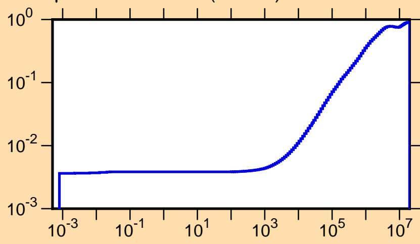
\mu vs. E for ^{186}\text{Au}(\text{mt251})
