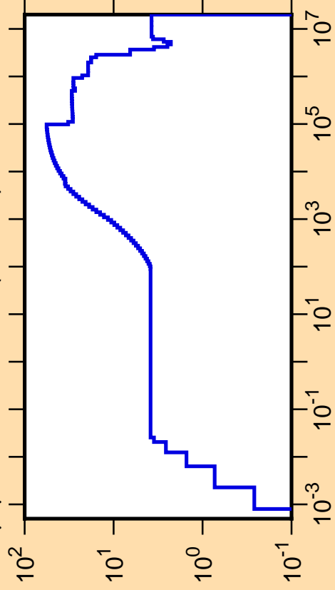
\Delta\mu/\mu vs. E for ^{186}\text{Au}(\text{mt251})
