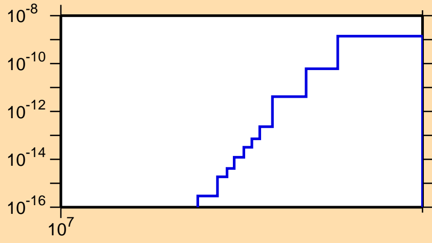
\sigma vs. E for ^{186}\text{Au}(n,\text{pt})
