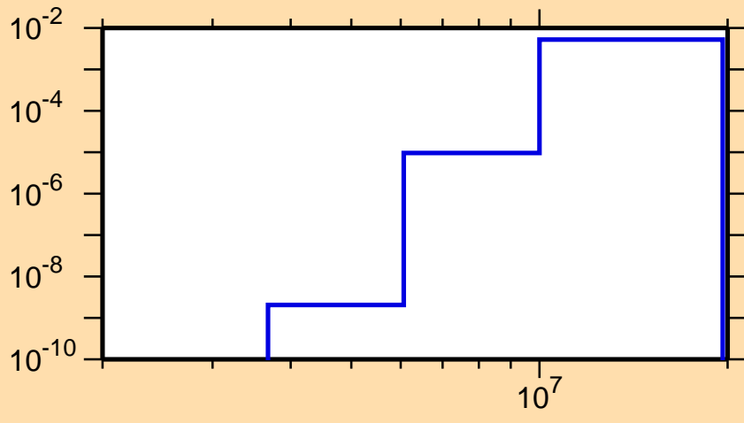
\sigma vs. E for ^{186}\text{Au}(n,d)
