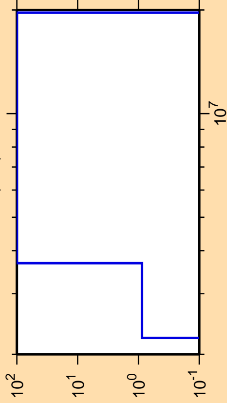
\Delta\sigma/\sigma vs. E for ^{186}\text{Au}(n,d)
