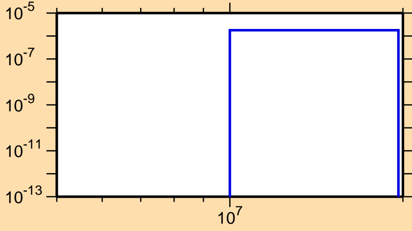
\sigma vs. E for ^{186}\text{Au}(n,\text{nd})
