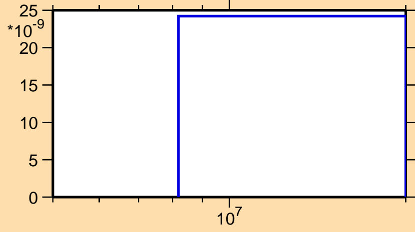
\sigma vs. E for ^{186}\text{Au}(\text{mt } 45)
