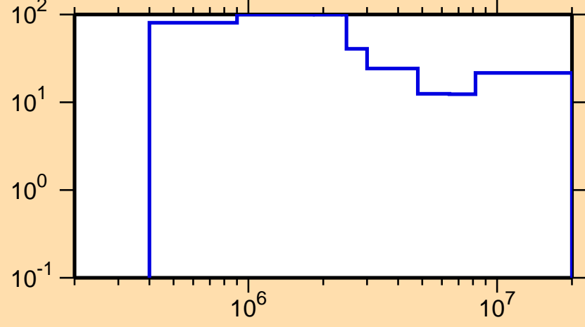
\Delta\sigma/\sigma vs. E for ^{186}\text{Au}(n,n\text{cont.})
