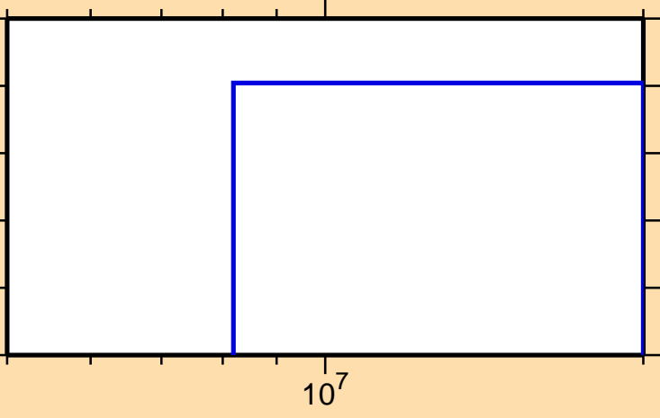
\sigma vs. E for ^{186}\text{Au}(n,\text{pd})
