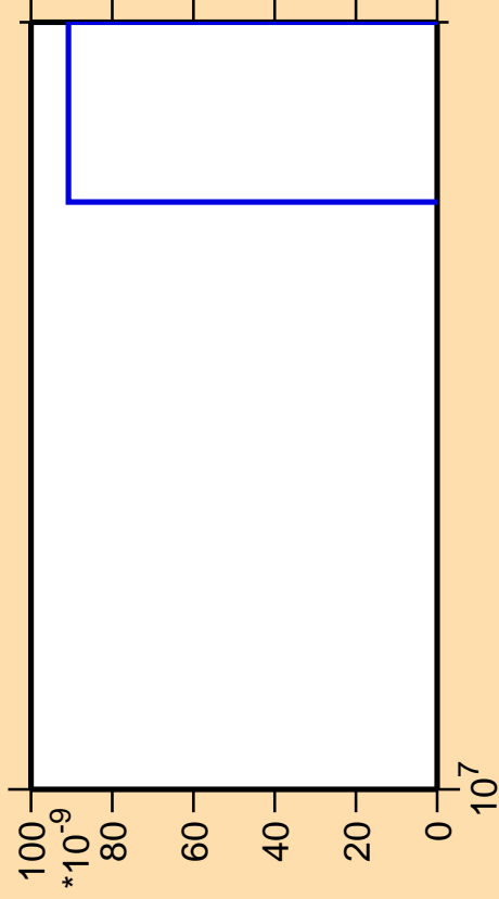
\Delta\sigma/\sigma vs. E for ^{187}\text{Au} (mt 42)
