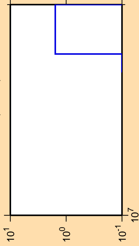
\Delta\sigma/\sigma vs. E for ^{187}\text{Au}(n,3n\alpha)
