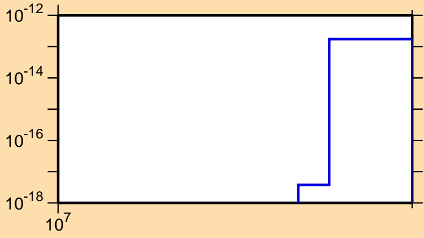
\sigma vs. E for ^{187}\text{Au}(n,3n\alpha)
