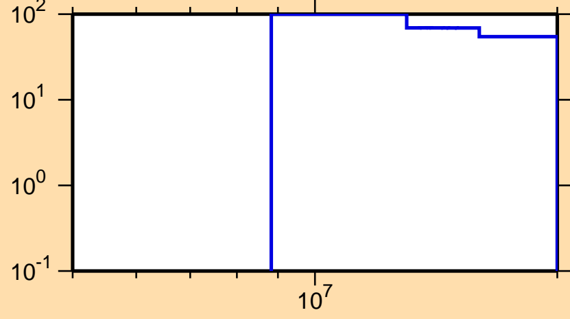
\Delta\sigma/\sigma vs. E for ^{187}\text{Au}(n,2n)
