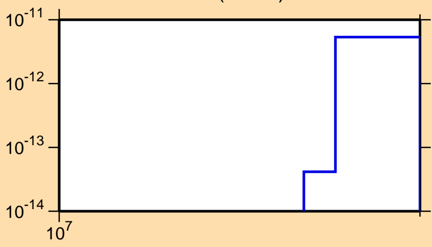
\sigma vs. E for ^{187}\text{Au}(\text{mt } 34)
