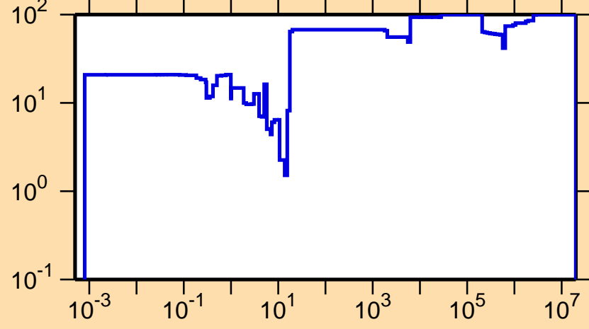
\Delta\sigma/\sigma vs. E for ^{187}\text{Au}(n,\gamma)
