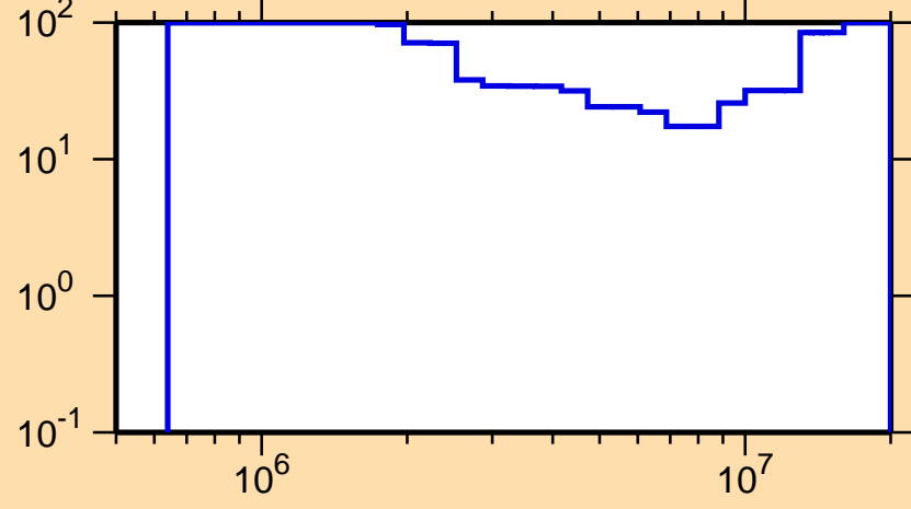
\Delta\sigma/\sigma vs. E for ^{187}\text{Au}(n,ncont.)
