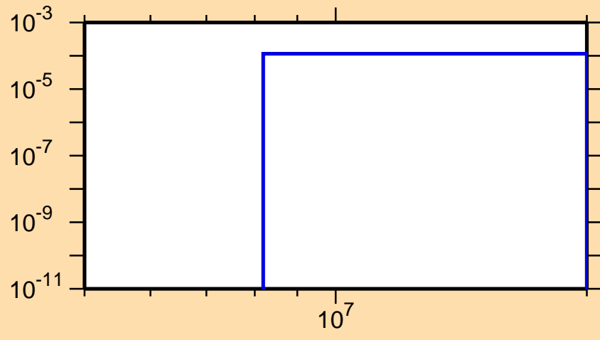
\sigma vs. E for ^{187}\text{Au}(n,t)
