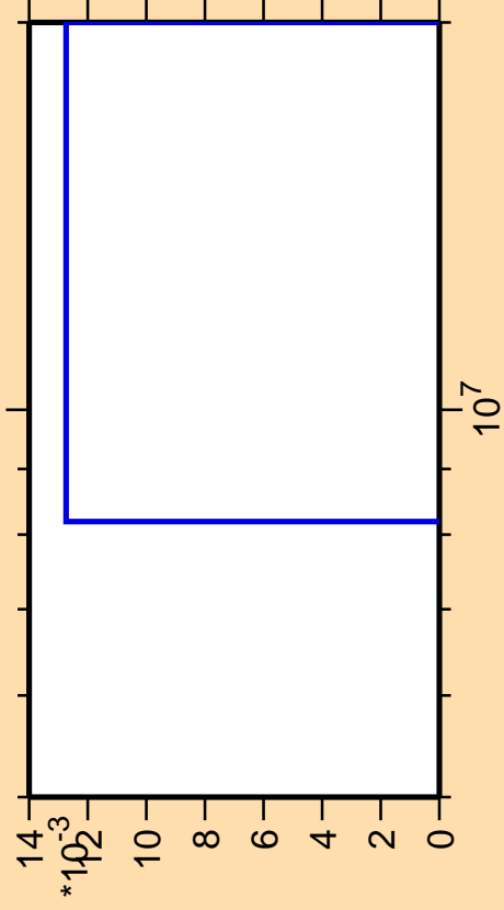
\Delta\sigma/\sigma vs. E for ^{187}\text{Au}(n,3n\alpha)
