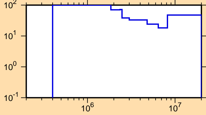
\Delta\sigma/\sigma vs. E for ^{187}\text{Au}(n,n\text{cont.})
