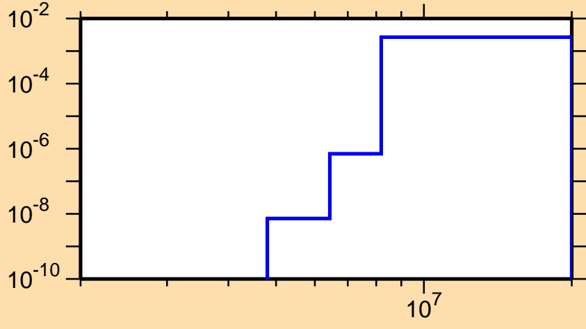
\sigma vs. E for ^{187}\text{Au}(n,d)
