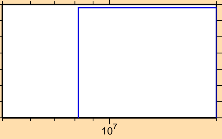
\sigma vs. E for ^{187}\text{Au}(n,3n)
