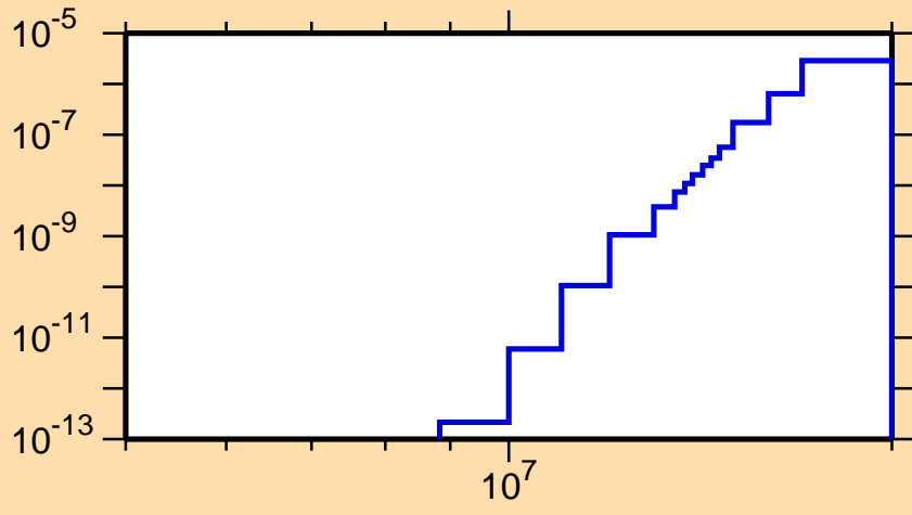
\sigma vs. E for ^{187}\text{Au}(n,\text{He3})
