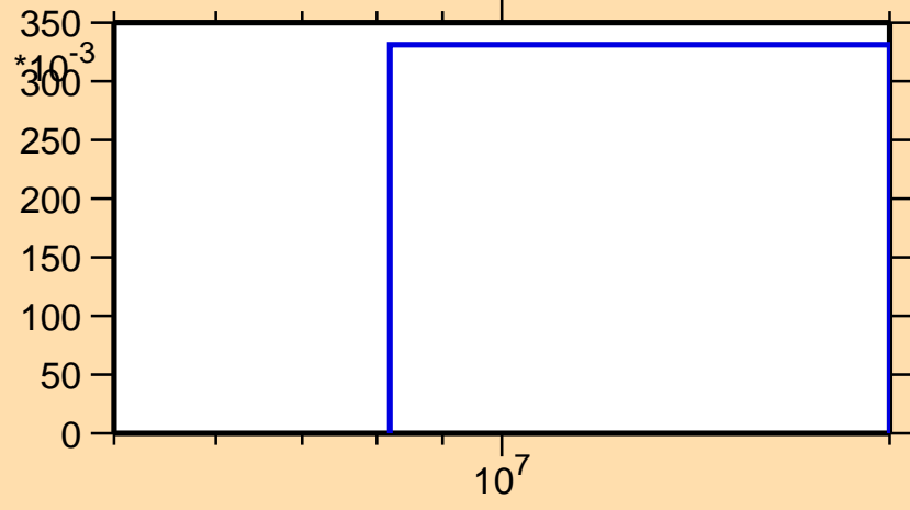
\sigma vs. E for ^{187}\text{Au}(n,2n)
