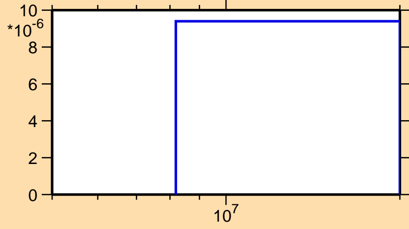
\sigma vs. E for ^{187}\text{Au}(n,3n)
