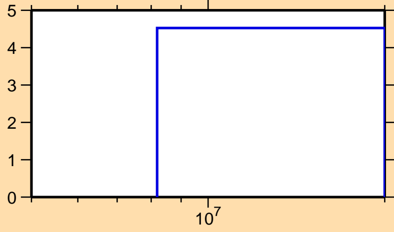
\Delta\sigma/\sigma vs. E for ^{187}\text{Au}(n,\text{el.})
