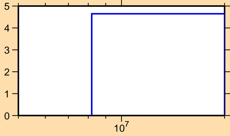
\Delta\sigma/\sigma vs. E for ^{187}\text{Au}(n,\text{tot.})
