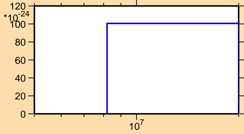
\sigma vs. E for ^{187}\text{Au}(\text{mt } 42)
