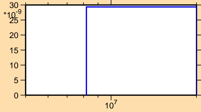
\sigma vs. E for ^{187}\text{Au}(n,\text{nd})
