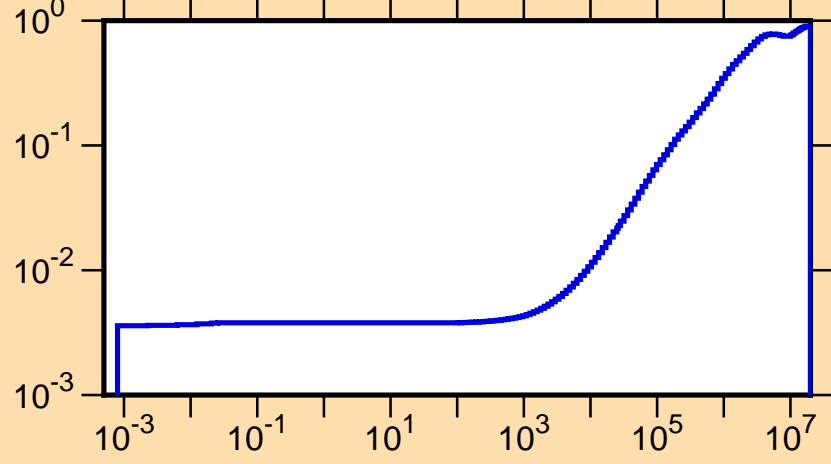
\mu vs. E for ^{188}\text{Au}(\text{mt251})
