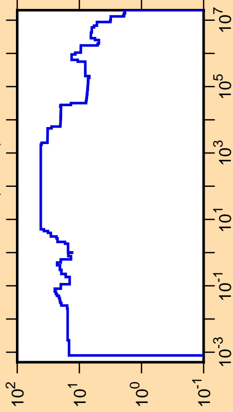
\Delta\sigma/\sigma vs. E for ^{188}\text{Au}(n,\text{tot.})
