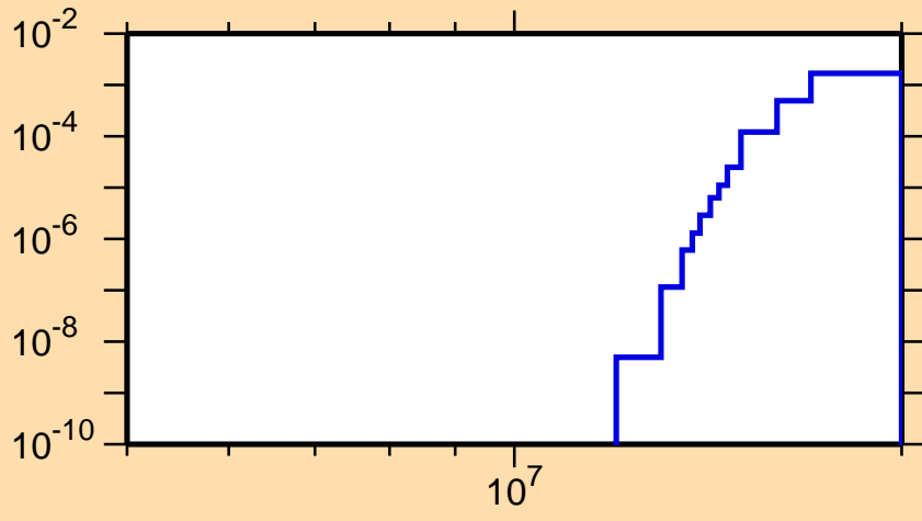
\sigma vs. E for ^{188}\text{Au}(n,2np)
