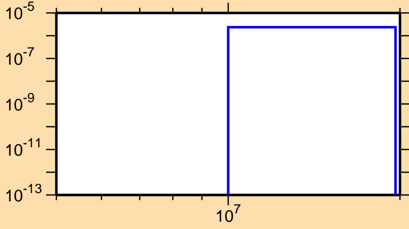
\sigma vs. E for ^{188}\text{Au}(n,\text{nd})
