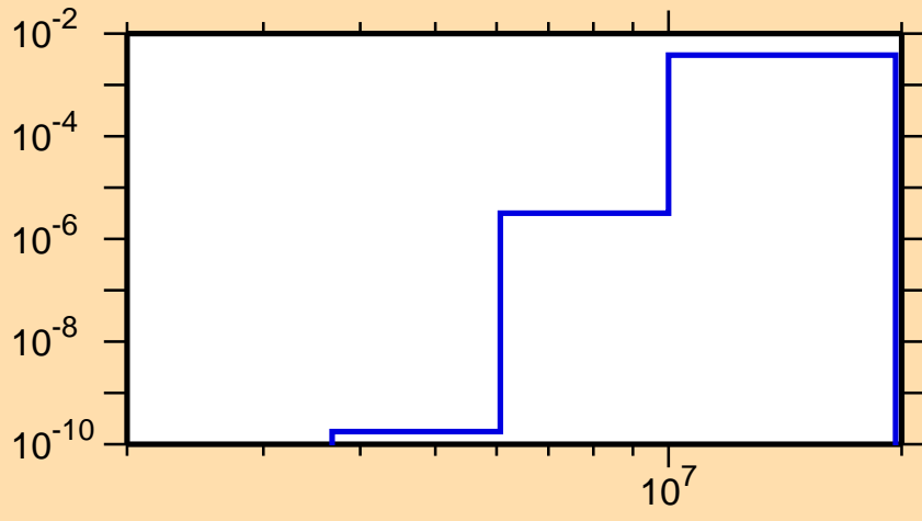
\sigma vs. E for ^{188}\text{Au}(n,d)
