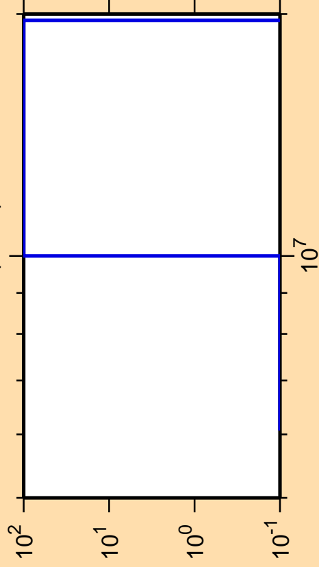
\Delta\sigma/\sigma vs. E for ^{188}\text{Au}(n,\text{nd})
