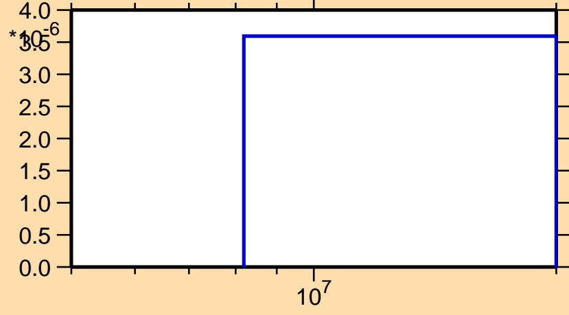
\sigma vs. E for ^{188}\text{Au}(n,2n\alpha)
