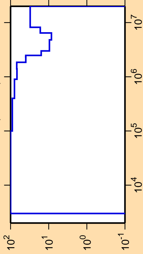
\Delta\sigma/\sigma vs. E for ^{188}\text{Au}(n,\text{inel.})
