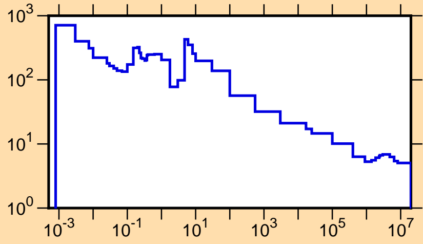
\sigma vs. E for ^{188}\text{Au}(n,\text{tot.})
