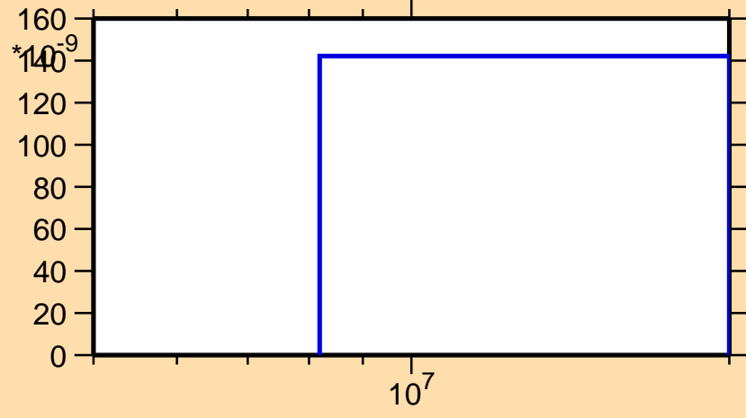
\sigma vs. E for ^{188}\text{Au}(n,\text{He}3)
