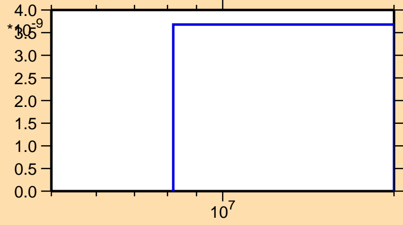
\sigma vs. E for ^{188}\text{Au}(\text{mt } 45)
