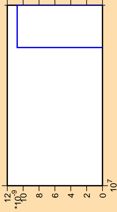
\Delta\sigma/\sigma vs. E for ^{189}\text{Au}(\text{mt } 42)
