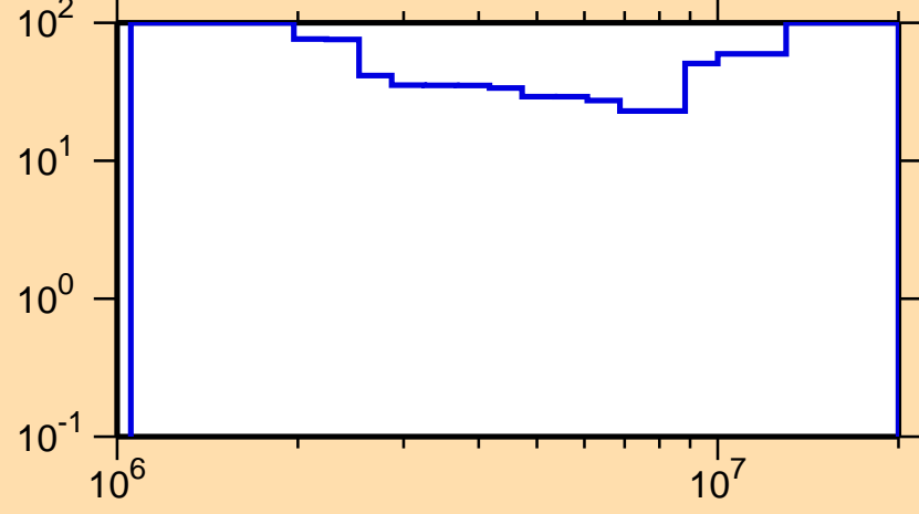
\Delta\sigma/\sigma vs. E for ^{189}\text{Au}(n,n\text{cont.})
