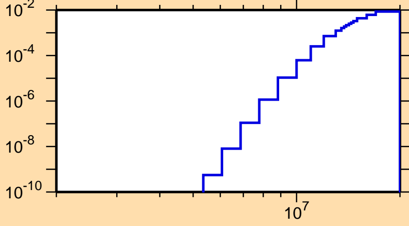
\sigma vs. E for ^{189}\text{Au}(n,d)
