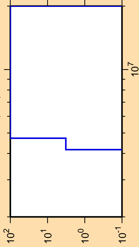
\Delta\sigma/\sigma vs. E for ^{189}\text{Au}(n,d)
