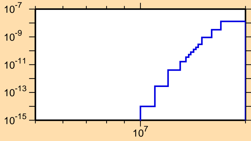
\sigma vs. E for ^{189}\text{Au}(\text{mt } 45)
