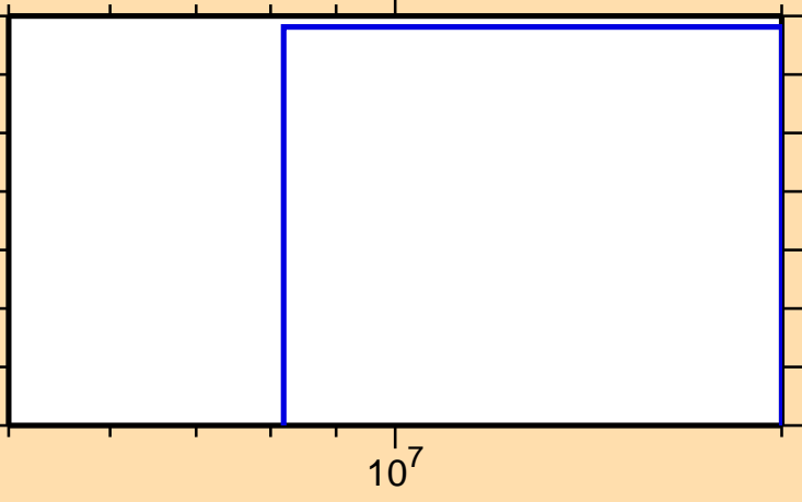
\sigma vs. E for ^{189}\text{Au}(n,3n)
