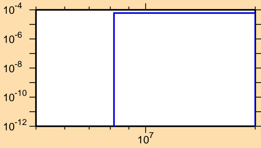
\sigma vs. E for ^{189}\text{Au}(n,t)
