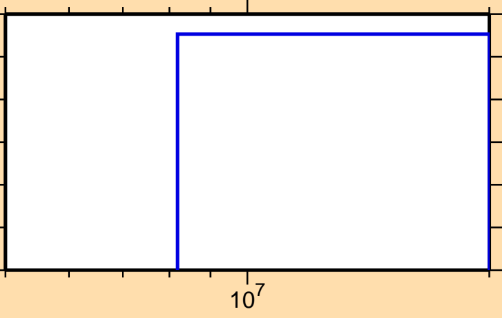
\sigma vs. E for ^{189}\text{Au}(n,\text{nd})
