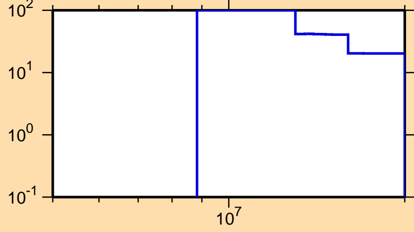
\Delta\sigma/\sigma vs. E for ^{189}\text{Au}(n,2n)
