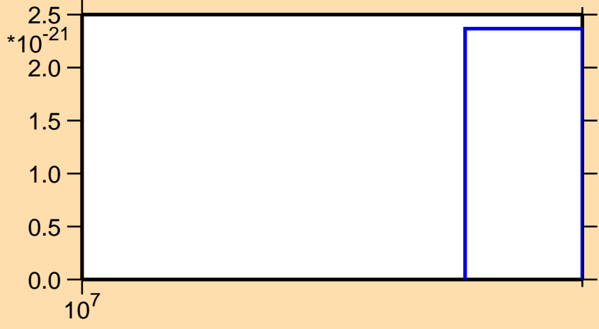
\sigma vs. E for ^{189}\text{Au}(\text{mt } 42)
