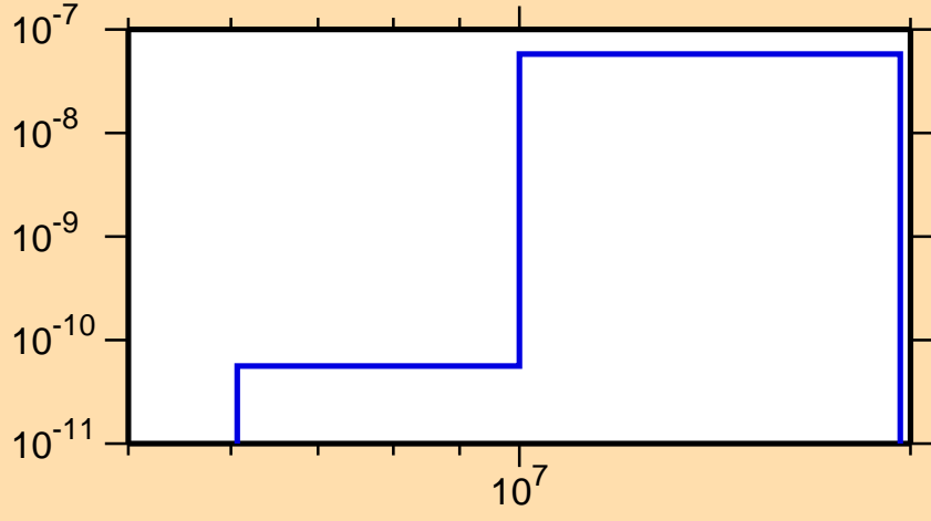
\sigma vs. E for ^{189}\text{Au}(n,p\alpha)
