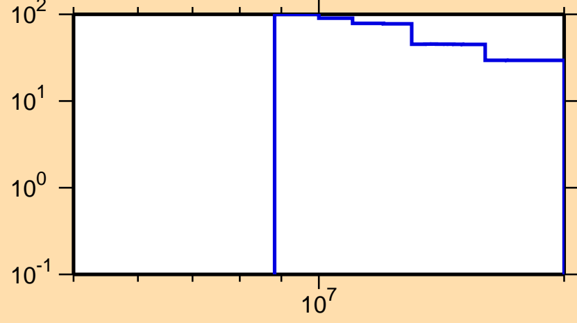
\Delta\sigma/\sigma vs. E for ^{191}\text{Au}(n,2n)
