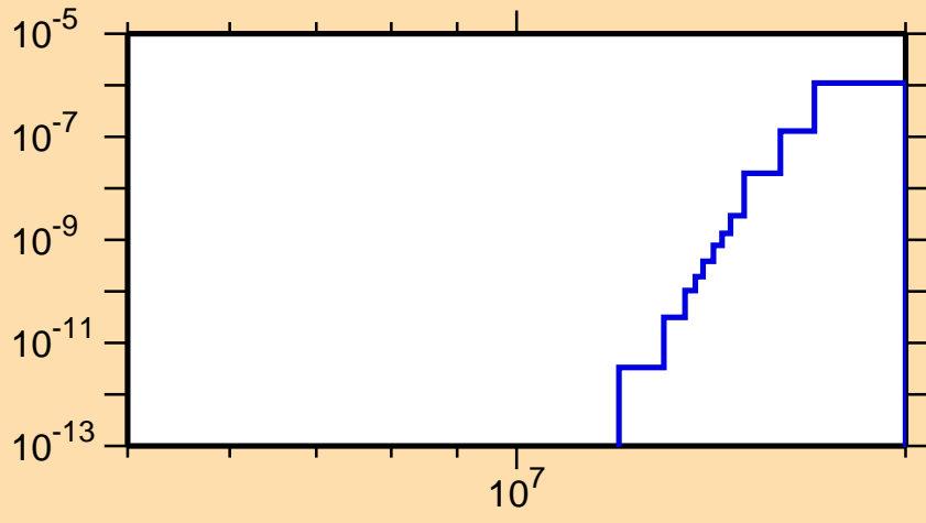
\sigma vs. E for ^{191}\text{Au}(n,2n\alpha)
