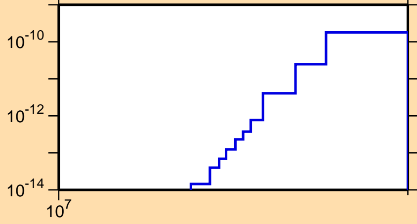
\sigma vs. E for ^{191}\text{Au}(\text{mt } 45)
