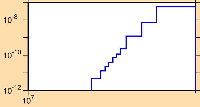
\sigma vs. E for ^{191}\text{Au}(n,\text{He3})
