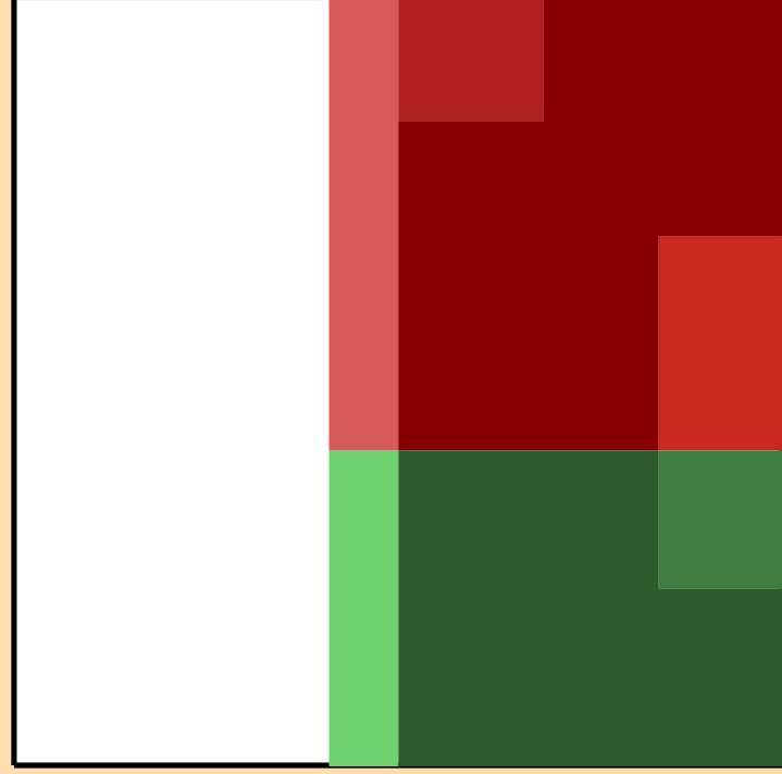
\Delta\sigma/\sigma vs. E for ^{191}\text{Au}(n,2n)
