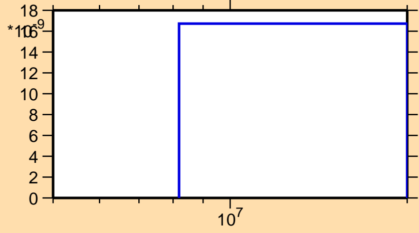
\sigma vs. E for ^{191}\text{Au}(n,2n\alpha)
