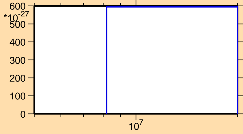
\sigma vs. E for ^{191}\text{Au}(\text{mt } 42)
