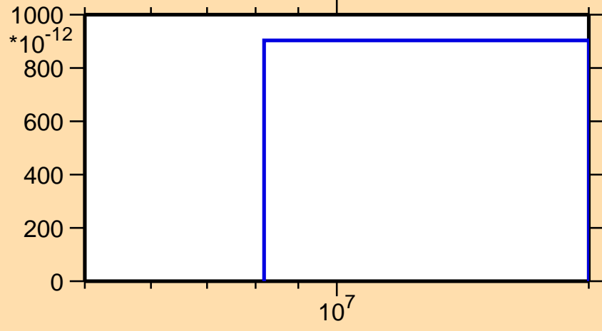
\sigma vs. E for ^{191}\text{Au}(n,\text{He3})
