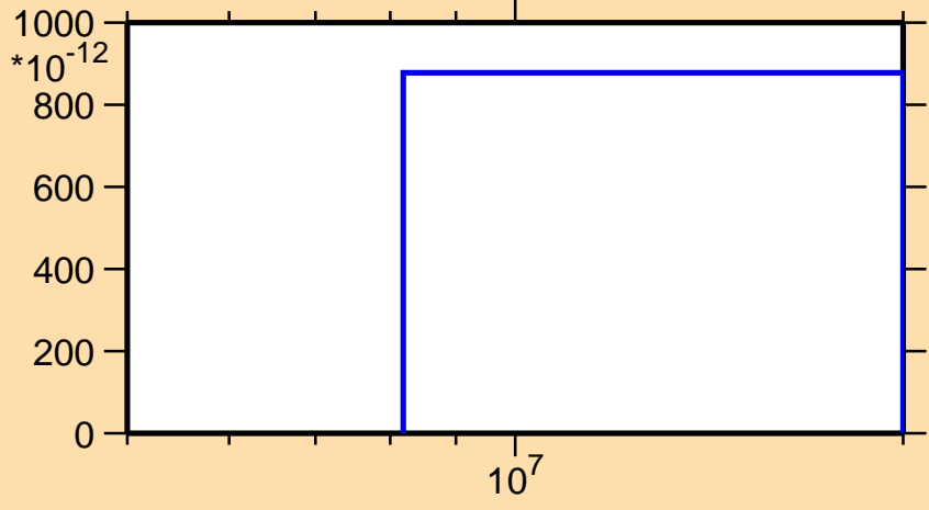
\sigma vs. E for ^{191}\text{Au}(n,nt)
