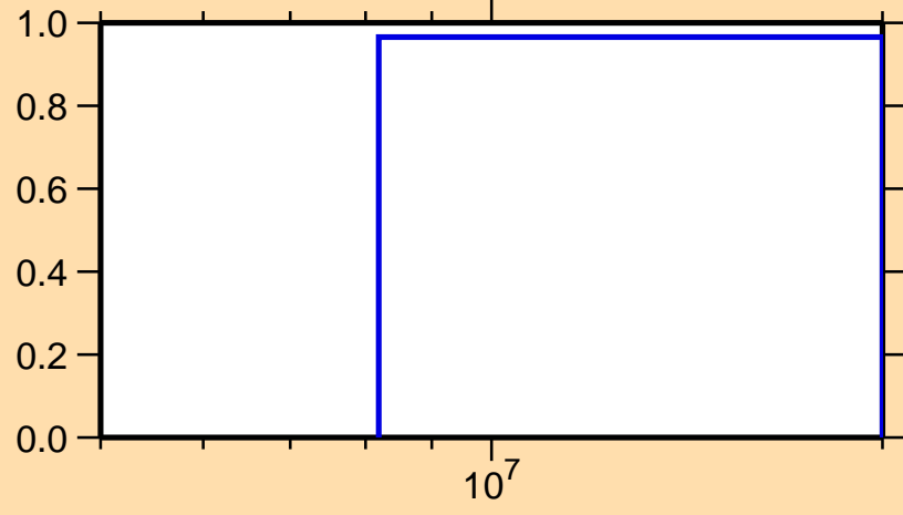
\sigma vs. E for ^{191}\text{Au}(n,2n)
