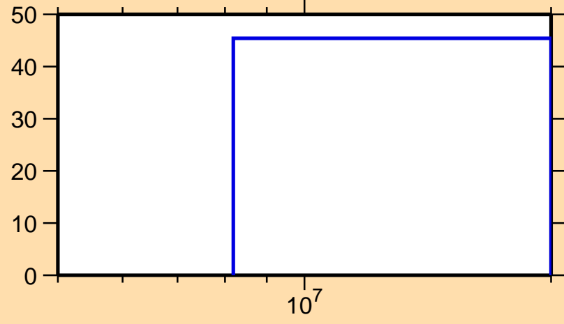
\Delta\sigma/\sigma vs. E for ^{191}\text{Au}(n,2n)
