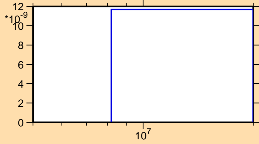
\sigma vs. E for ^{191}\text{Au}(n,\text{nd})
