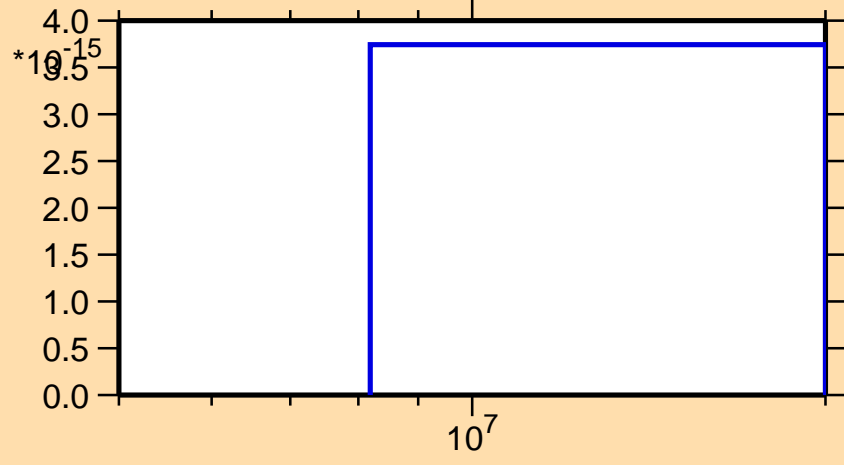
\sigma vs. E for ^{191}\text{Au}(n,\text{pd})
