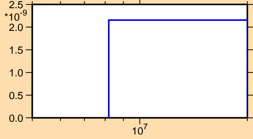
\sigma vs. E for ^{191}\text{Au}(n,p\alpha)
