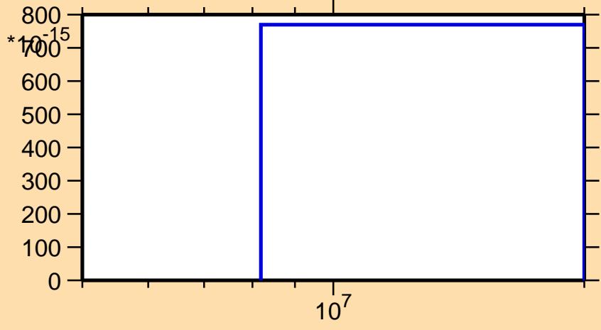
\sigma vs. E for ^{191}\text{Au}(\text{mt117})
