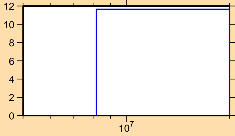
\Delta\sigma/\sigma vs. E for ^{191}\text{Au}(n,\text{el.})
