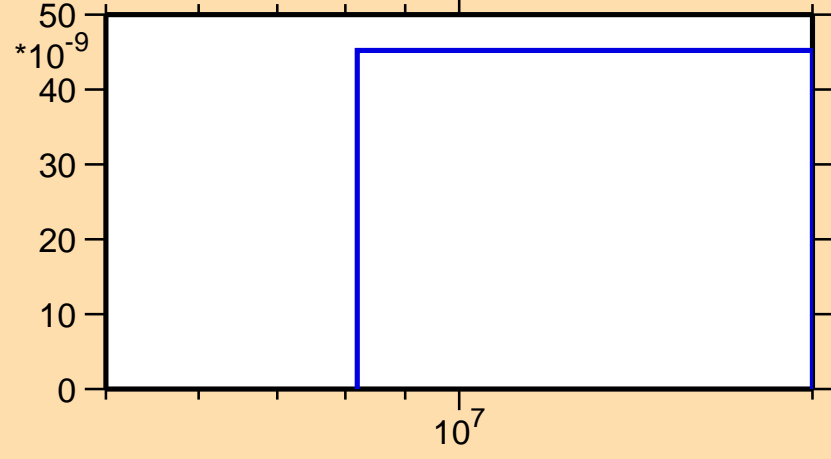
\sigma vs. E for ^{191}\text{Au}(n,2np)
