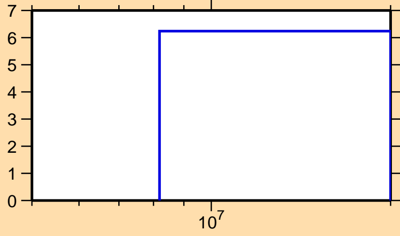
\Delta\sigma/\sigma vs. E for ^{191}\text{Au}(n,\text{tot.})
