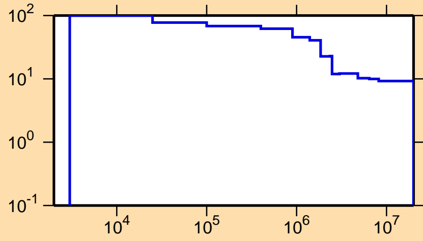
\Delta\sigma/\sigma vs. E for ^{191}\text{Au}(n,\text{nonel.})
