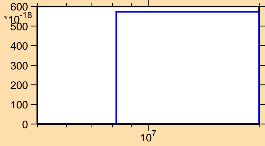
\sigma vs. E for ^{191}\text{Au}(n,3n\alpha)
