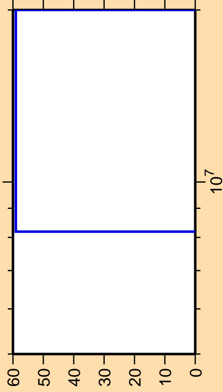
\Delta\sigma/\sigma vs. E for ^{191}\text{Au}(n,n\text{cont.})
