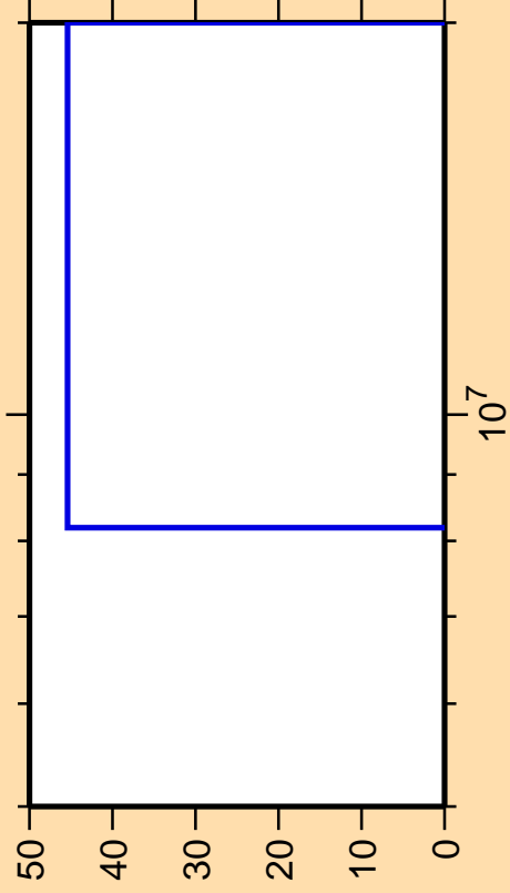
\Delta\sigma/\sigma vs. E for ^{191}\text{Au}(n,2n)
