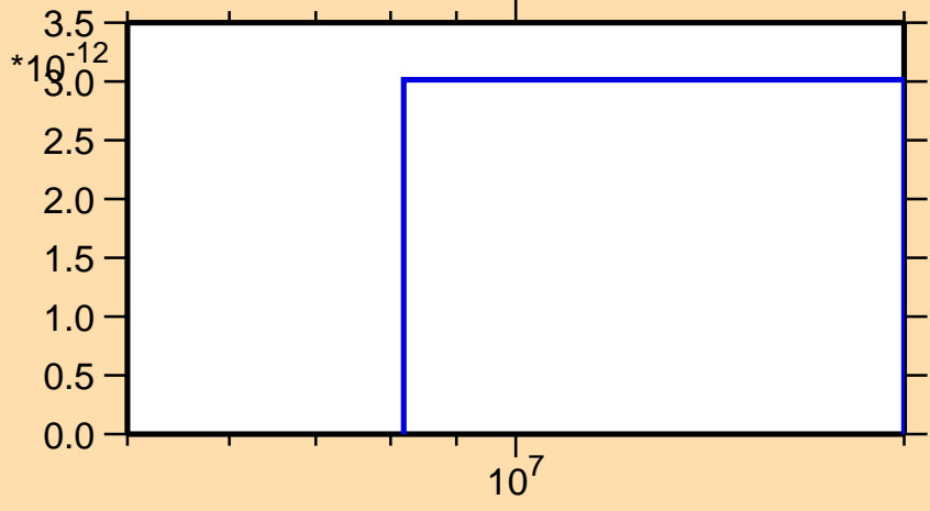
\sigma vs. E for ^{191}\text{Au}(\text{mt } 45)
