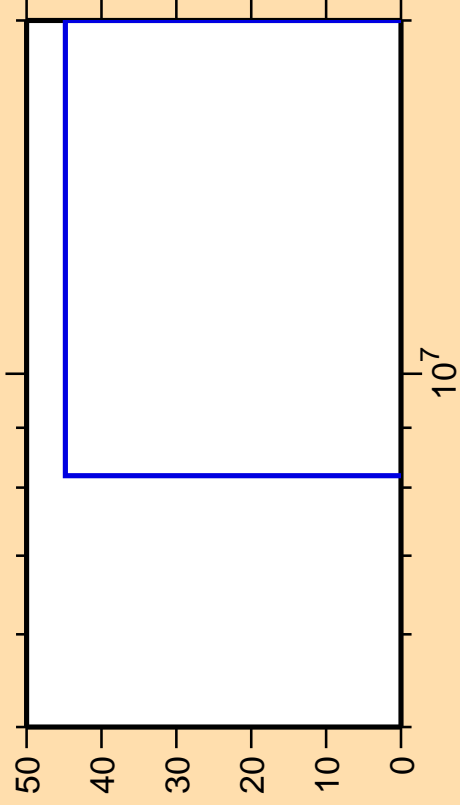
\Delta\sigma/\sigma vs. E for ^{191}\text{Au}(n,n_1)
