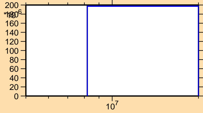
\sigma vs. E for ^{191}\text{Au}(n,3n)
