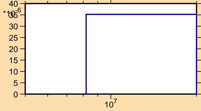
\sigma vs. E for ^{191}\text{Au}(n,t)
