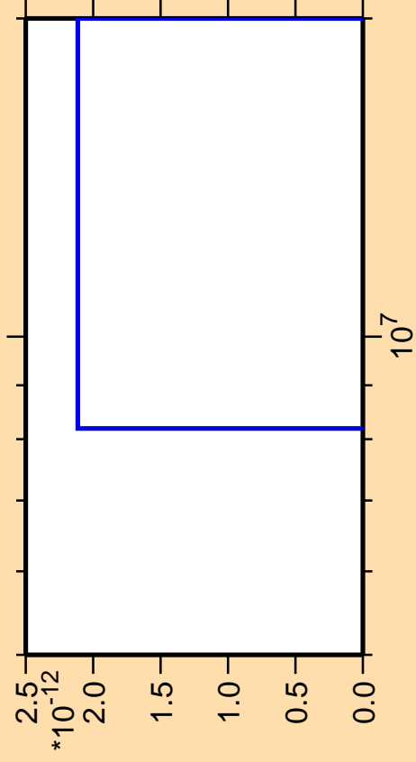
\Delta\sigma/\sigma vs. E for ^{191}\text{Au}(\text{mt } 42)
