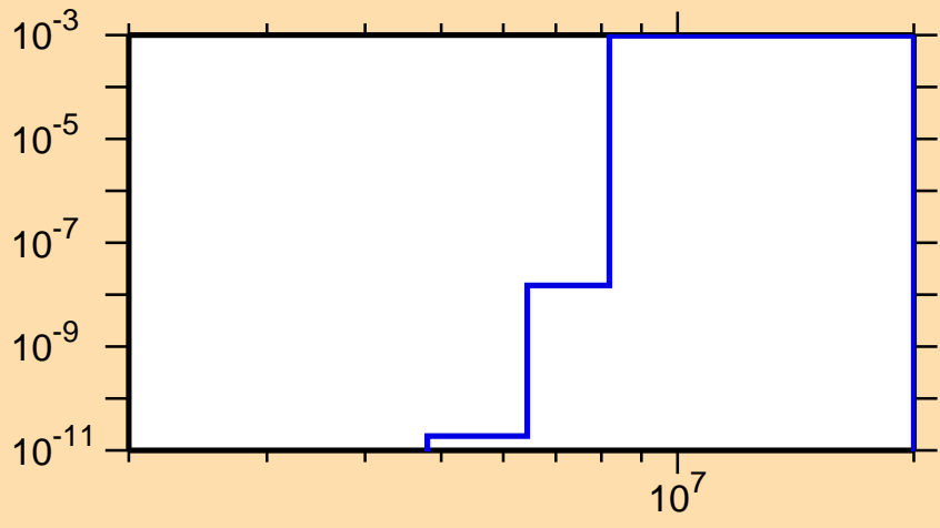
\sigma vs. E for ^{191}\text{Au}(n,d)
