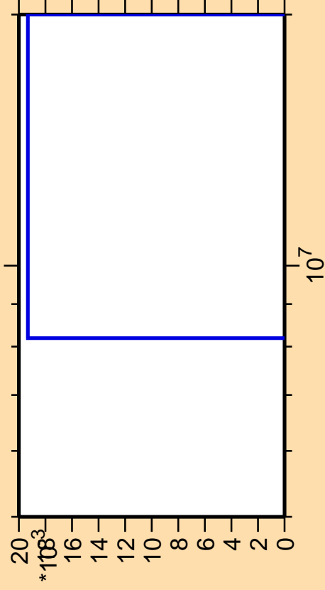
\Delta\sigma/\sigma vs. E for ^{191}\text{Au}(n,\text{pd})
