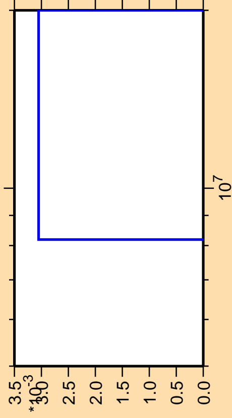
\Delta\sigma/\sigma vs. E for ^{191}\text{Au}(n,3n\alpha)
