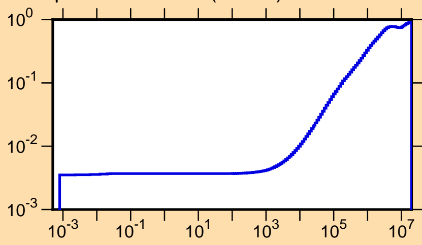
\mu vs. E for ^{192}\text{Au}(\text{mt251})
