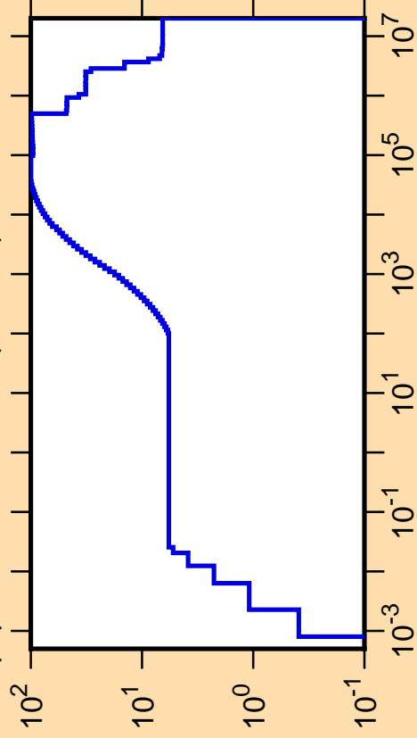
\Delta\mu/\mu vs. E for ^{192}\text{Au}(\text{mt251})
