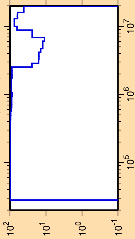
\Delta\sigma/\sigma vs. E for ^{192}\text{Au}(n,\text{inel.})
