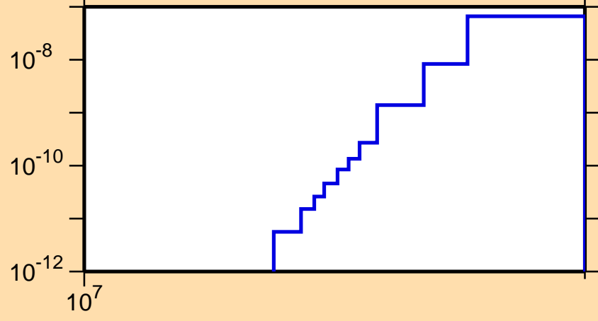
\sigma vs. E for ^{192}\text{Au}(n,\text{He3})
