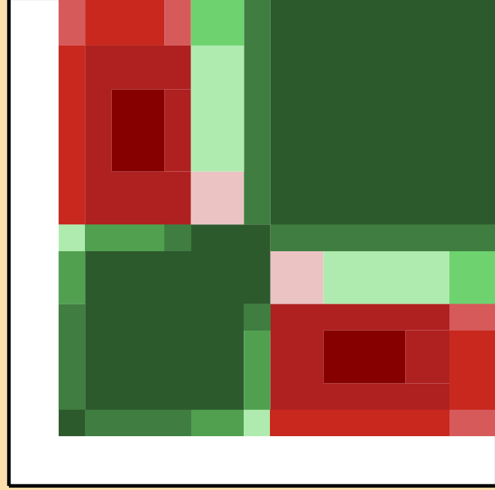
\sigma vs. E for ^{192}\text{Au}(n,n\text{cont.})
