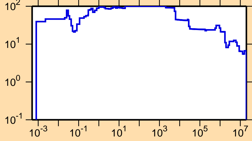
\Delta\sigma/\sigma vs. E for ^{192}\text{Au}(n,\text{tot.})
