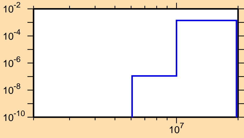
\sigma vs. E for ^{192}\text{Au}(n,d)
