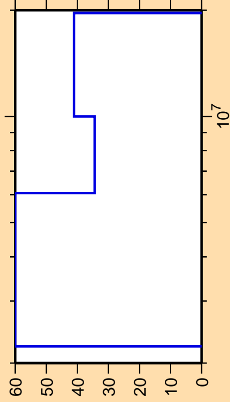
\Delta\sigma/\sigma vs. E for ^{192}\text{Au}(n,p)
