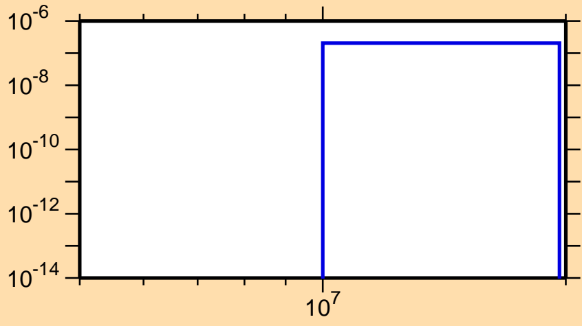
\sigma vs. E for ^{192}\text{Au}(n,2n\alpha)
