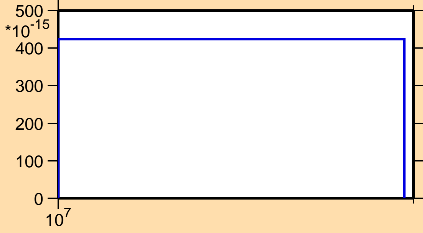
\sigma vs. E for ^{192}\text{Au}(\text{mt } 45)
