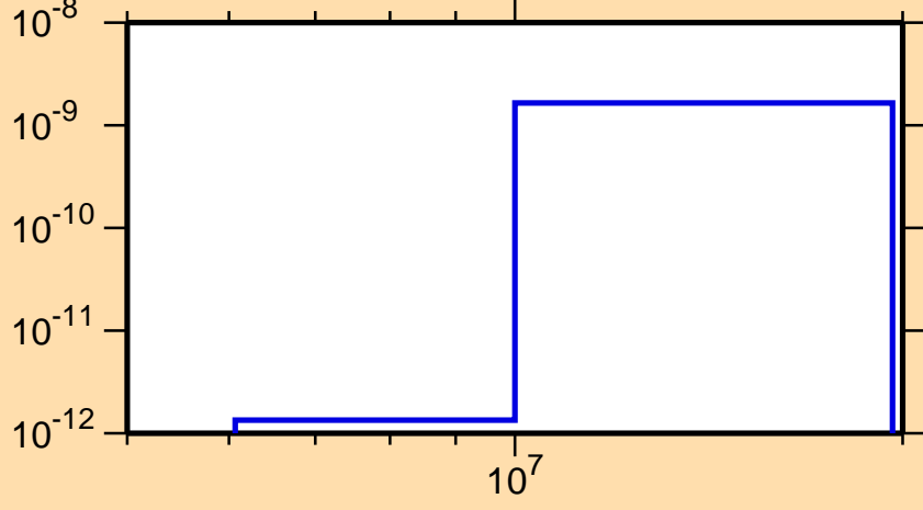
\sigma vs. E for ^{192}\text{Au}(n,p\alpha)
