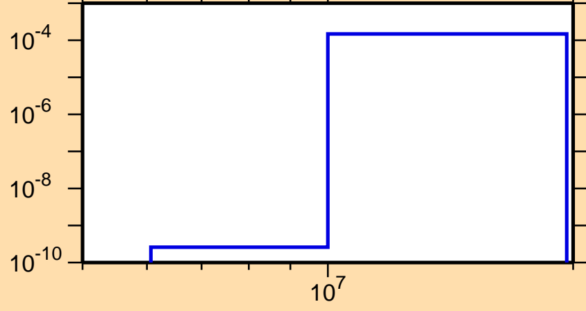
\sigma vs. E for ^{192}\text{Au}(n,t)
