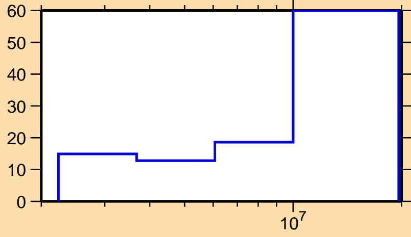
\Delta\sigma/\sigma vs. E for ^{192}\text{Au}(n,ncont.)
