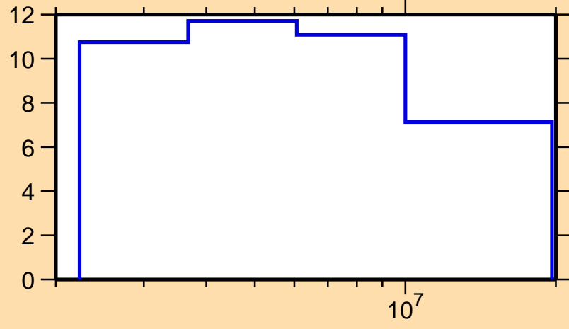
\Delta\sigma/\sigma vs. E for ^{192}\text{Au}(n,n\text{nonel.})
