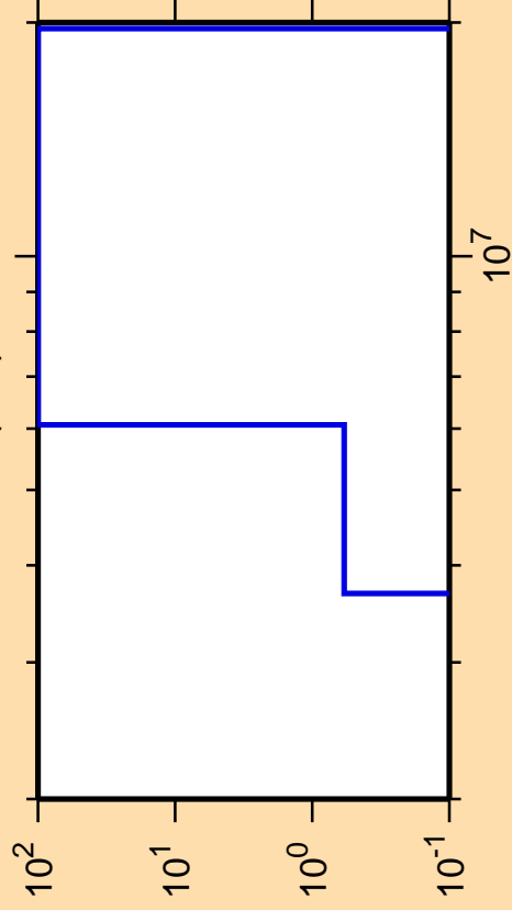
\Delta\sigma/\sigma vs. E for ^{192}\text{Au}(n,d)
