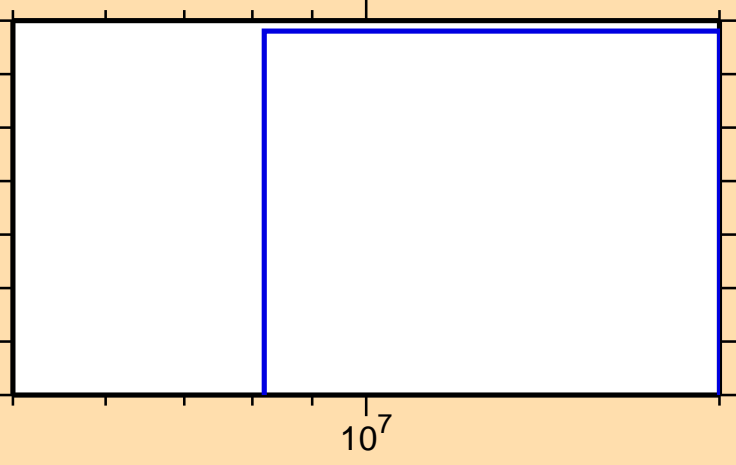
\sigma vs. E for ^{192}\text{Au}(n,\text{nd})
