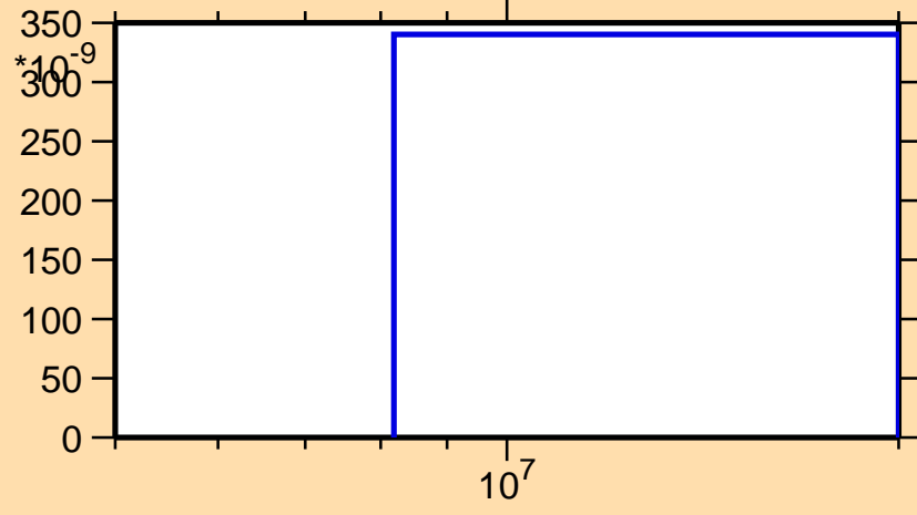
\sigma vs. E for ^{192}\text{Au}(n,\text{nd})
