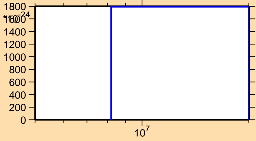
\sigma vs. E for ^{192}\text{Au}(\text{mt } 42)
