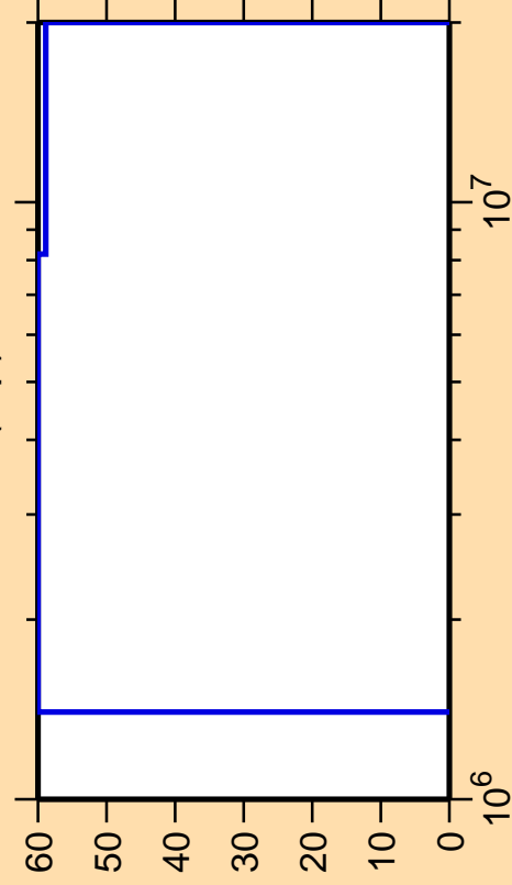
\Delta\sigma/\sigma vs. E for ^{193}\text{Au}(n,p)
