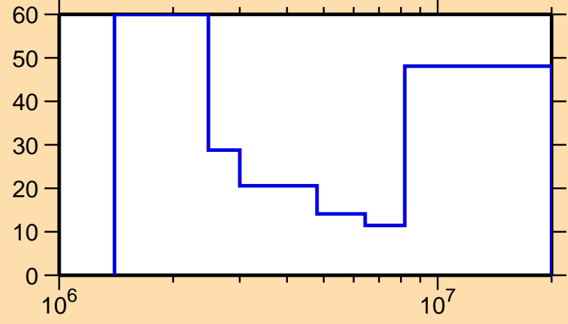
\Delta\sigma/\sigma vs. E for ^{193}\text{Au}(n,ncont.)
