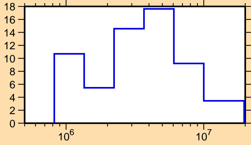
\Delta\sigma/\sigma vs. E for ^{193}\text{Au}(n,el.)
