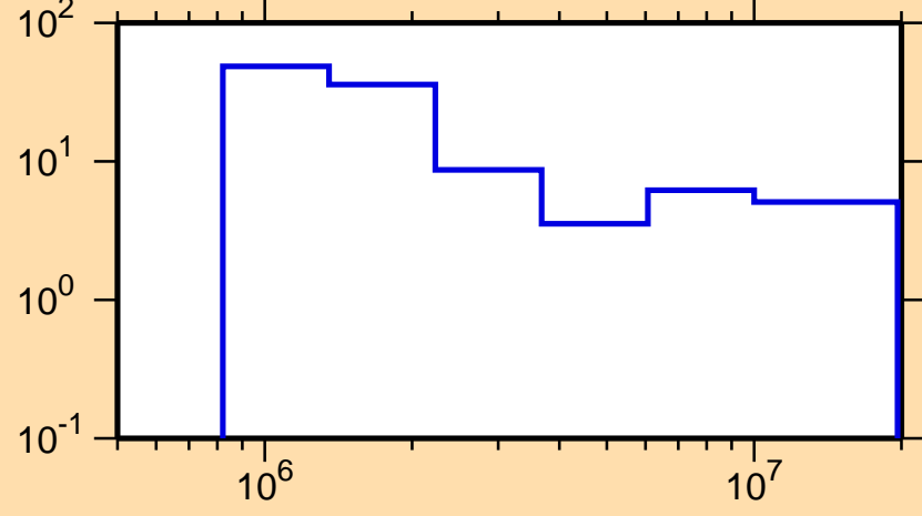
\Delta\sigma/\sigma vs. E for ^{193}\text{Au}(n,\text{nonel.})
