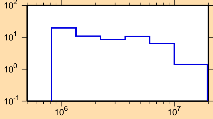
\Delta\sigma/\sigma vs. E for ^{193}\text{Au}(n,\text{tot.})
