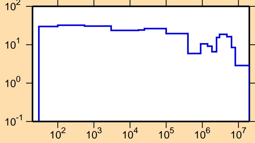
\Delta\sigma/\sigma vs. E for ^{193}\text{Au}(n,\text{el.})
