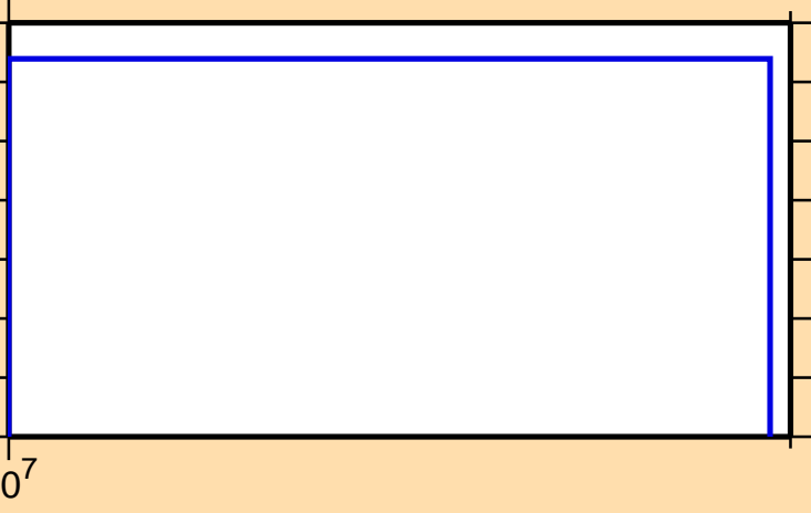
\sigma vs. E for ^{195}\text{Au}(n,3n)
