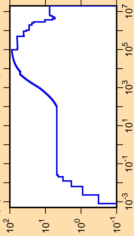
\Delta\mu/\mu vs. E for ^{196}\text{Au}(\text{mt251})
