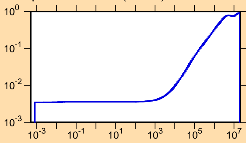
\mu vs. E for ^{196}\text{Au}(\text{mt251})
