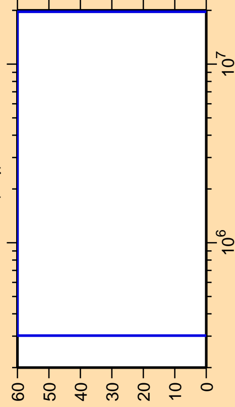
\Delta\sigma/\sigma vs. E for ^{196}\text{Au}(n,\gamma)
