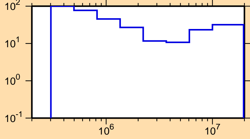
\Delta\sigma/\sigma vs. E for ^{196}\text{Au}(n,n\text{cont.})
