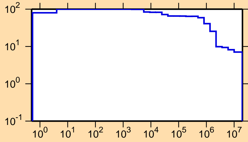
\Delta\sigma/\sigma vs. E for ^{196}\text{Au}(n,n\text{onel.})
