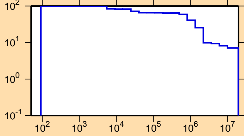
\Delta\sigma/\sigma vs. E for ^{196}\text{Au}(n,\text{nonel.})
