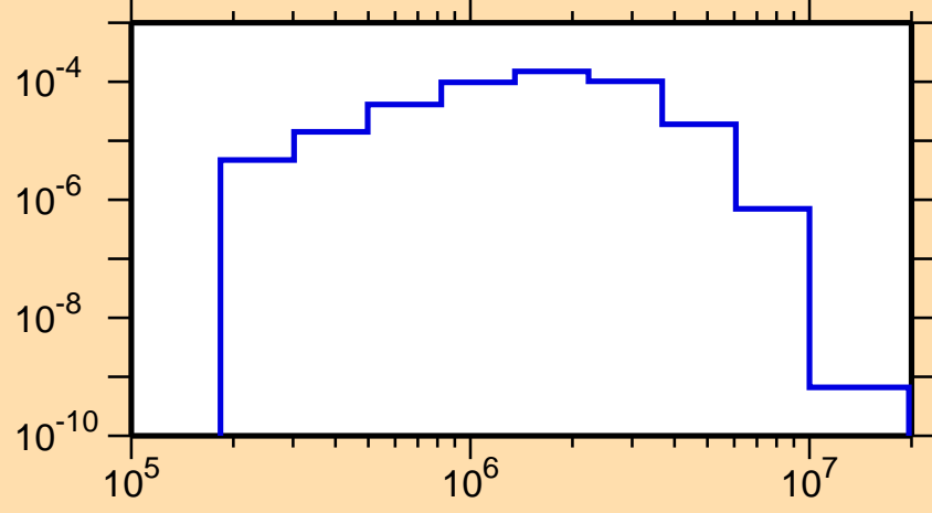
\sigma vs. E for ^{196}\text{Au}(n,n_4)
