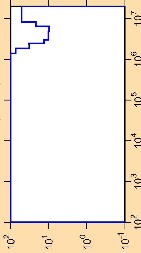
\Delta\sigma/\sigma vs. E for ^{196}\text{Au}(n,\text{inel.})
