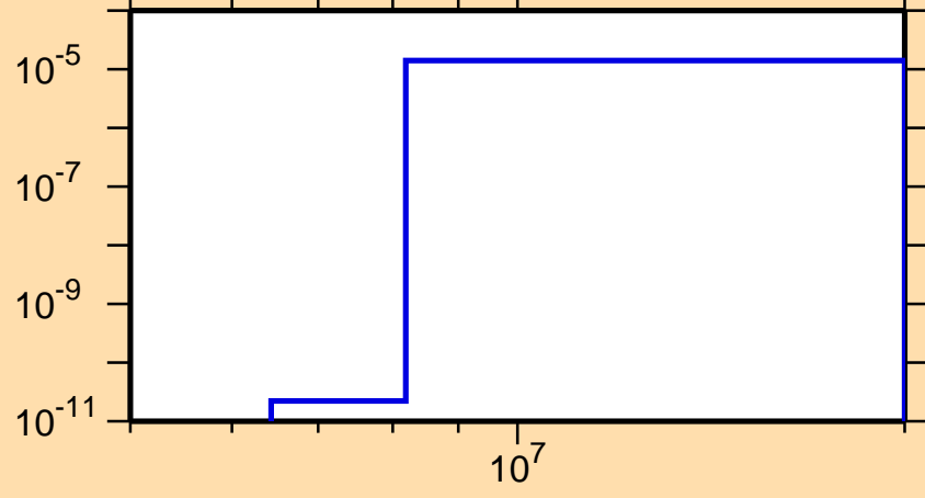
\sigma vs. E for ^{196}\text{Au}(n,n\alpha)
