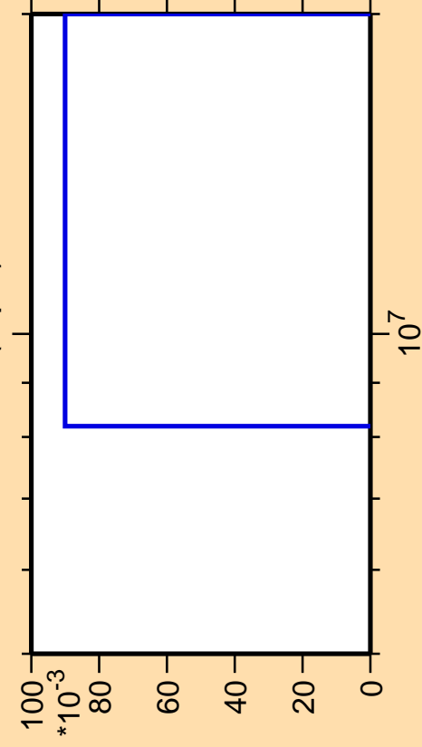
\Delta\sigma/\sigma vs. E for ^{196}\text{Au}(n,p\alpha)
