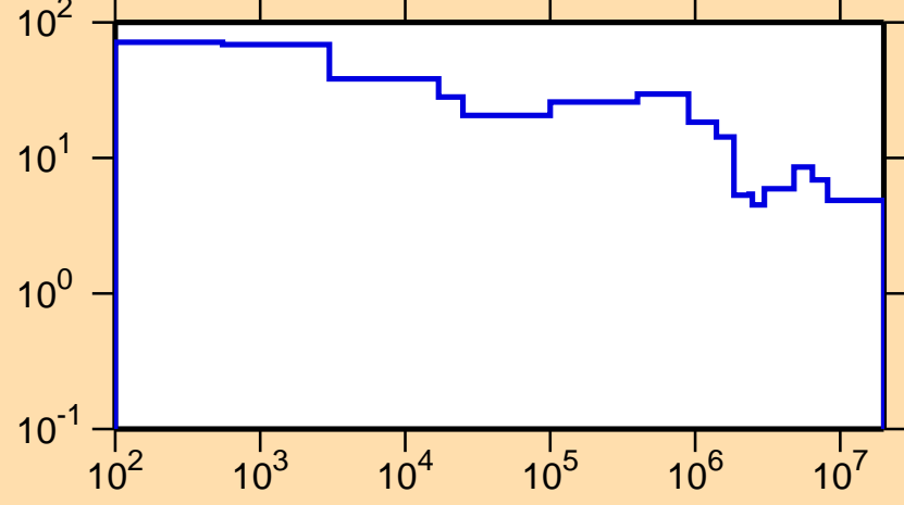
\Delta\sigma/\sigma vs. E for ^{196}\text{Au}(n,\text{tot.})
