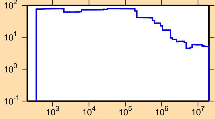
\Delta\sigma/\sigma vs. E for ^{197}\text{Au}(n,\text{nonel.})
