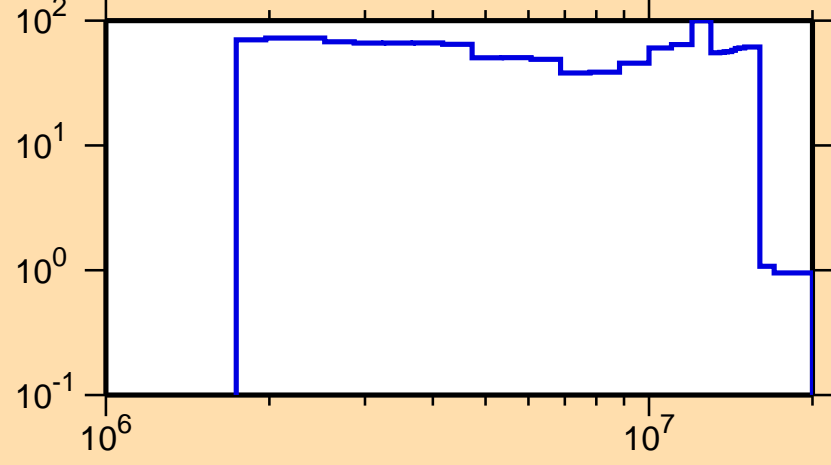
\Delta\sigma/\sigma vs. E for ^{197}\text{Au}(n,n_1)
