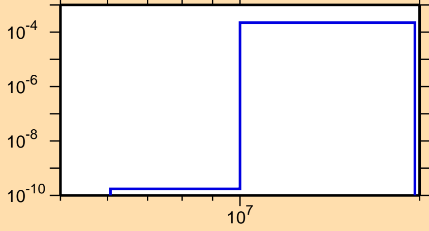
\sigma vs. E for ^{197}\text{Au}(n,d)
