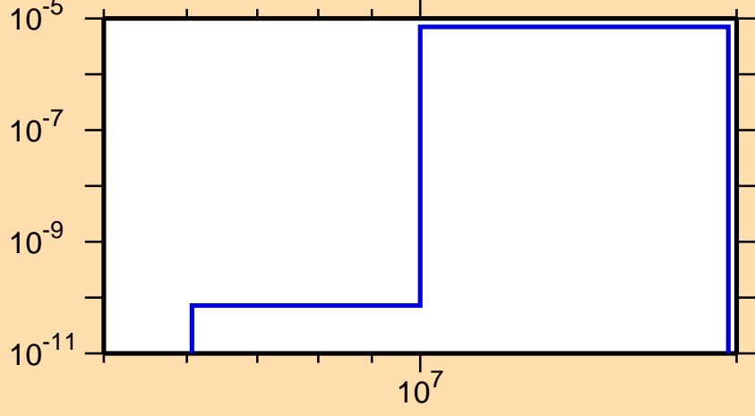
\sigma vs. E for ^{197}\text{Au}(n,n\alpha)
