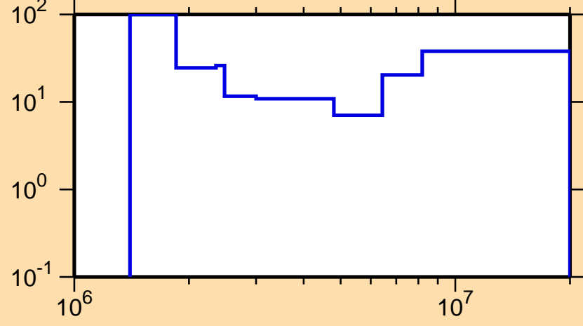
\Delta\sigma/\sigma vs. E for ^{197}\text{Au}(n,n\text{cont.})
