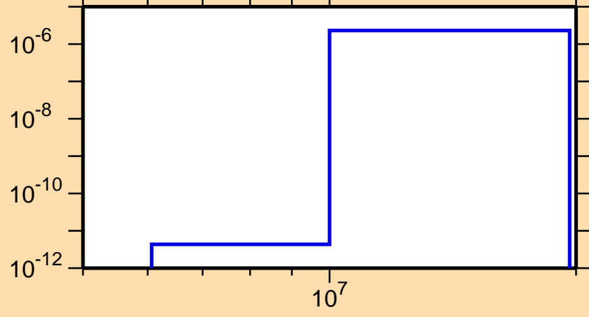
\sigma vs. E for ^{198}\text{Au}(n,n\alpha)
