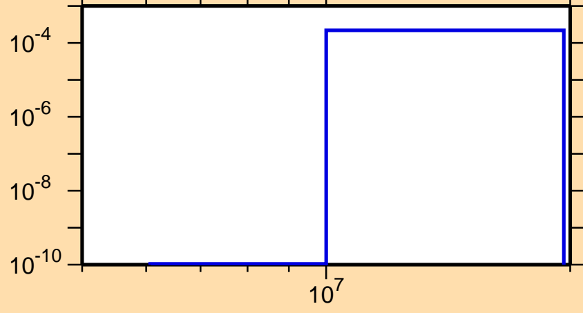
\sigma vs. E for ^{198}\text{Au}(n,d)
