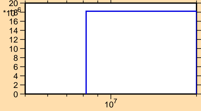
\sigma vs. E for ^{198}\text{Au}(n,t)
