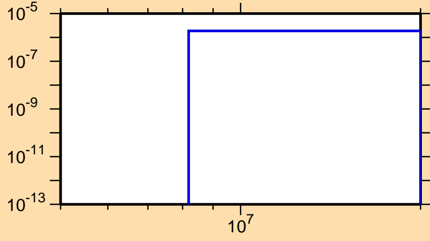
\sigma vs. E for ^{198}\text{Au}(n,n\alpha)
