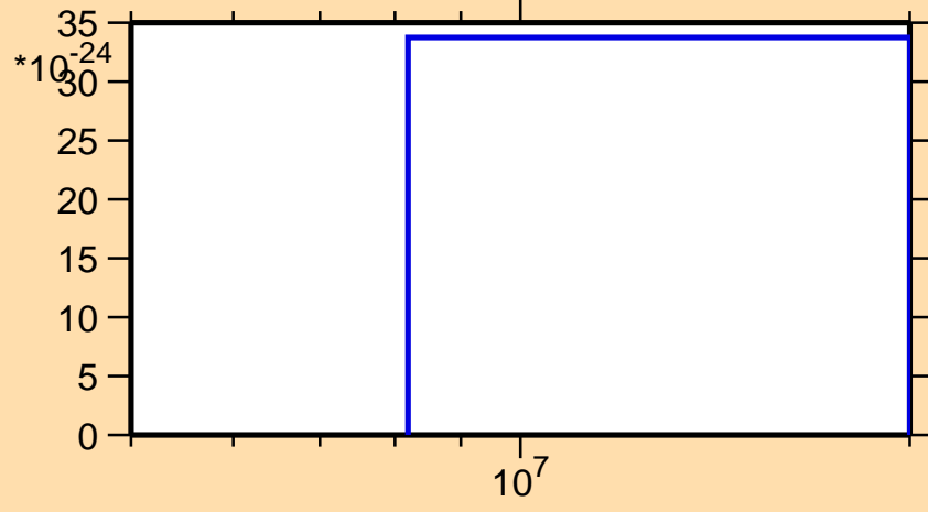
\sigma vs. E for ^{198}\text{Au}(\text{mt } 11)
