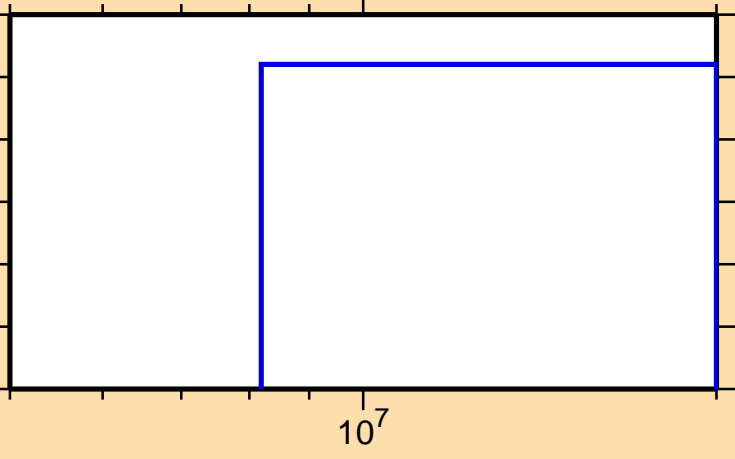
\sigma vs. E for ^{198}\text{Au}(n,2np)
