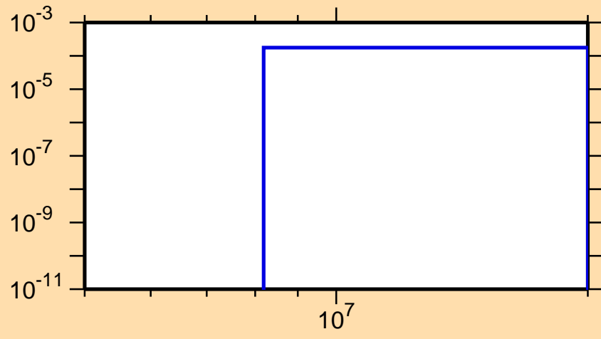
\sigma vs. E for ^{198}\text{Au}(n,d)
