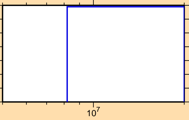
\sigma vs. E for ^{198}\text{Au}(n,np)
