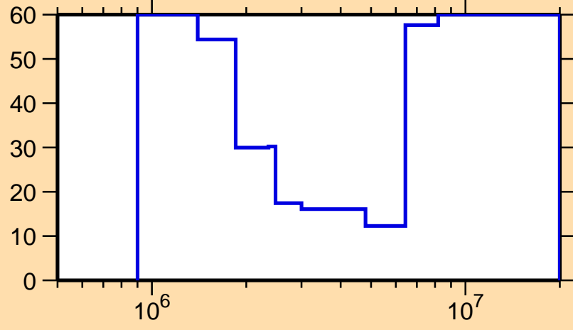
\Delta\sigma/\sigma vs. E for ^{198}\text{Au}(n,ncont.)
