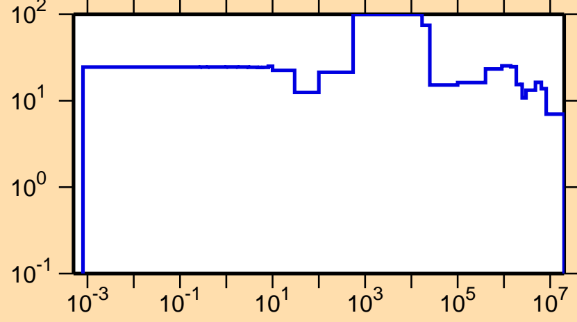
\Delta\sigma/\sigma vs. E for ^{198}\text{Au}(n,\text{el.})
