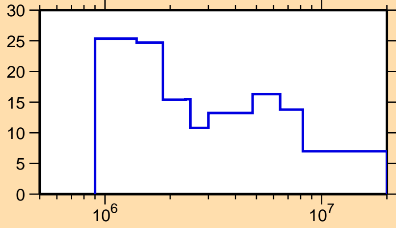
\Delta\sigma/\sigma vs. E for ^{198}\text{Au}(n,el.)
