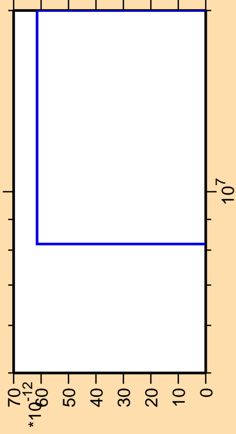
\Delta\sigma/\sigma vs. E for ^{198}\text{Au}(\text{mt } 11)
