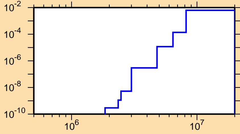
\sigma vs. E for ^{198}\text{Au}(n,p)
