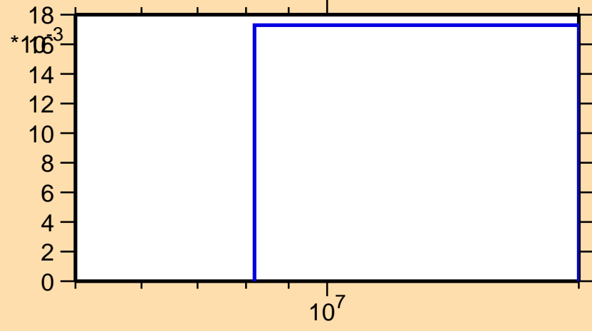
\sigma vs. E for ^{198}\text{Au}(n,3n)
