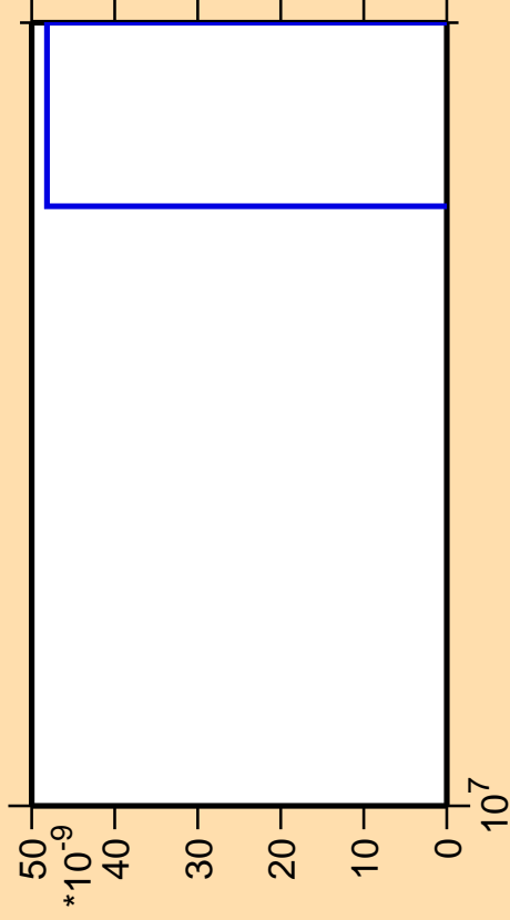
\Delta\sigma/\sigma vs. E for ^{199}\text{Au} (mt 42)
