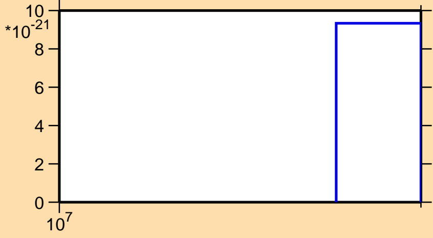
\sigma vs. E for ^{199}\text{Au} (mt 42)
