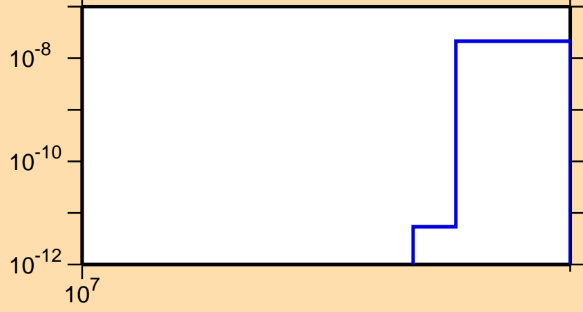
\sigma vs. E for ^{199}\text{Au}(n,2np)
