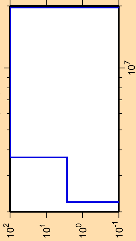
\Delta\sigma/\sigma vs. E for ^{199}\text{Au}(n,\alpha)
