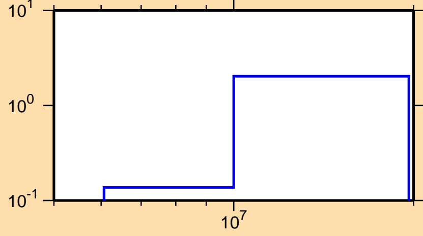
\sigma vs. E for ^{199}\text{Au}(n,2n)
