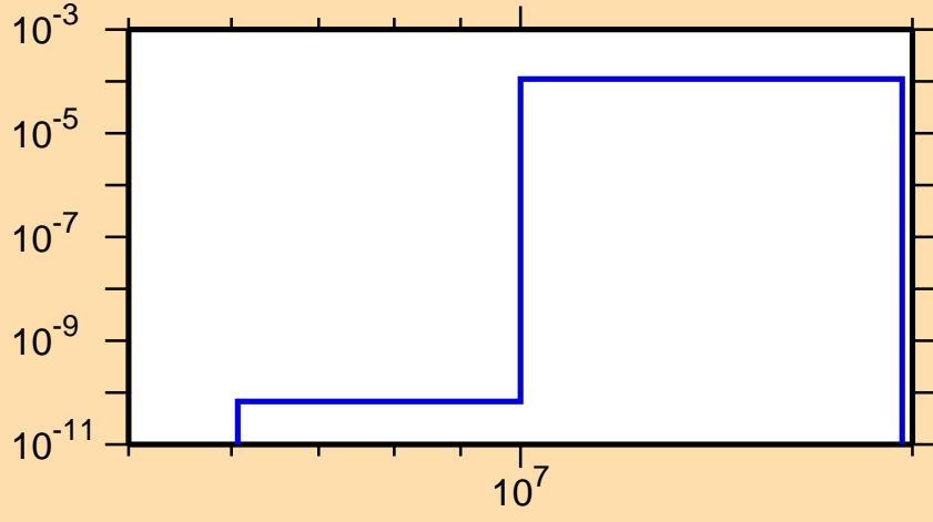
\sigma vs. E for ^{199}\text{Au}(n,d)
