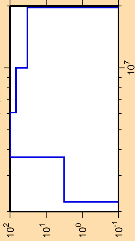
\Delta\sigma/\sigma vs. E for ^{199}\text{Au}(n,p)
