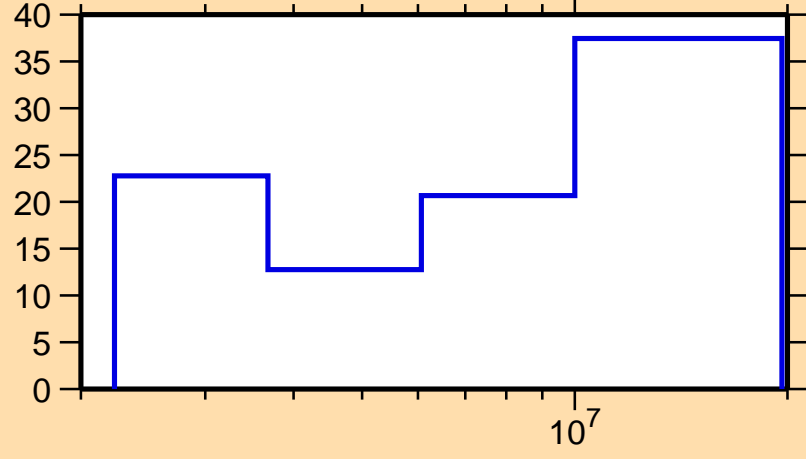
\Delta\sigma/\sigma vs. E for ^{199}\text{Au}(n,ncont.)
