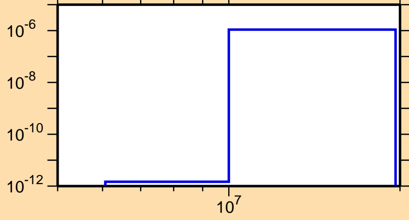
\sigma vs. E for ^{199}\text{Au}(n,n\alpha)
