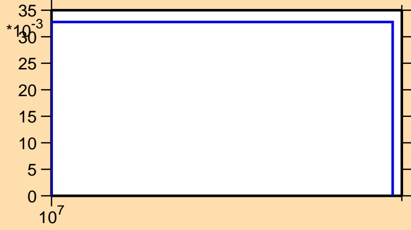
\sigma vs. E for ^{199}\text{Au}(n,3n)
