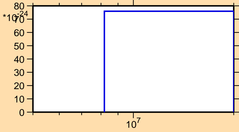
\sigma vs. E for ^{199}\text{Au}(\text{mt } 42)
