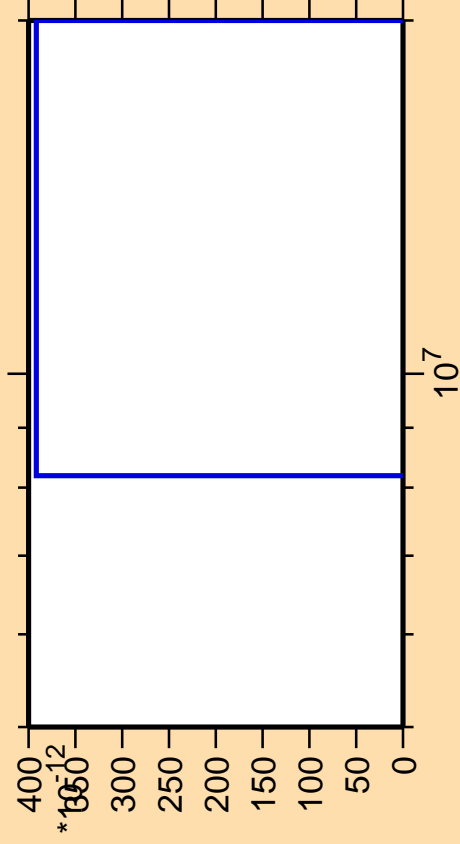
\Delta\sigma/\sigma vs. E for ^{199}\text{Au}(\text{mt } 42)
