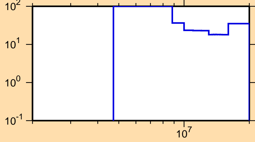
\Delta\sigma/\sigma vs. E for ^{200}\text{Au}(n,2n)
