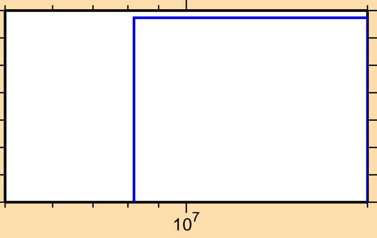
\sigma vs. E for ^{200}\text{Au}(n,n\alpha)
