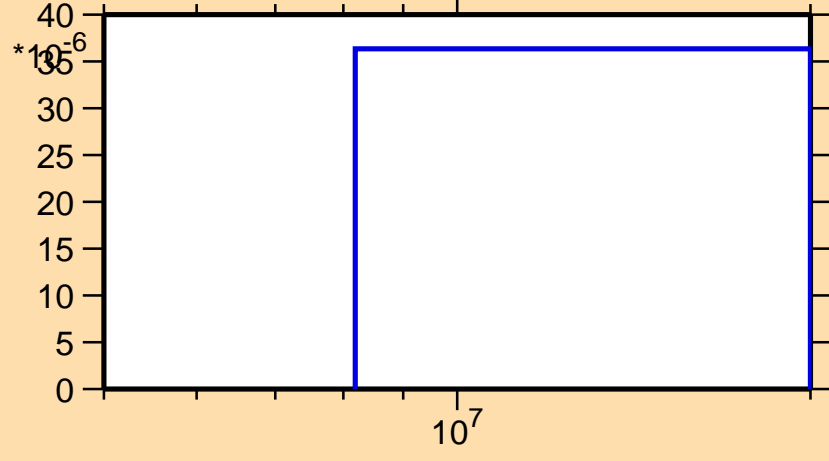
\sigma vs. E for ^{200}\text{Au}(n,t)
