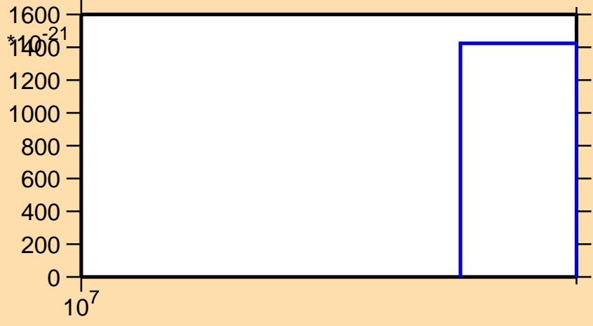
\sigma vs. E for ^{202}\text{Au}(\text{mt } 11)
