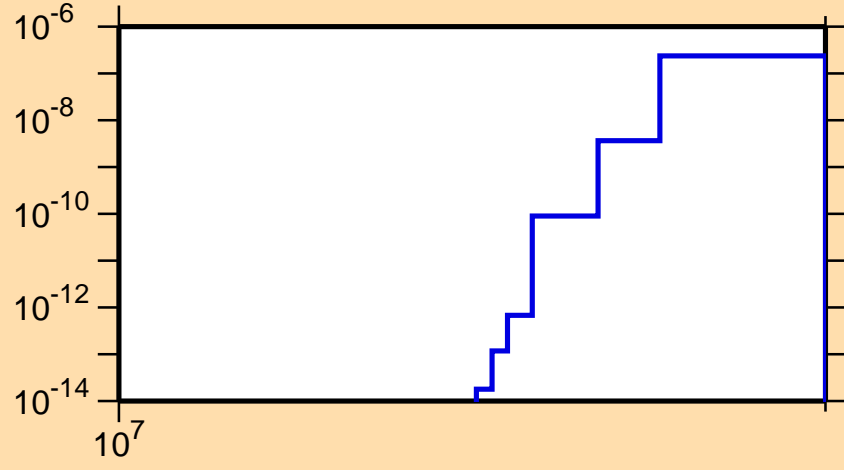
\sigma vs. E for ^{202}\text{Au}(n,\text{nd})
