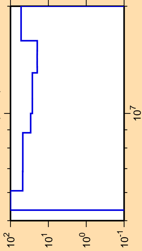
\Delta\sigma/\sigma vs. E for ^{202}\text{Au}(n,2n)
