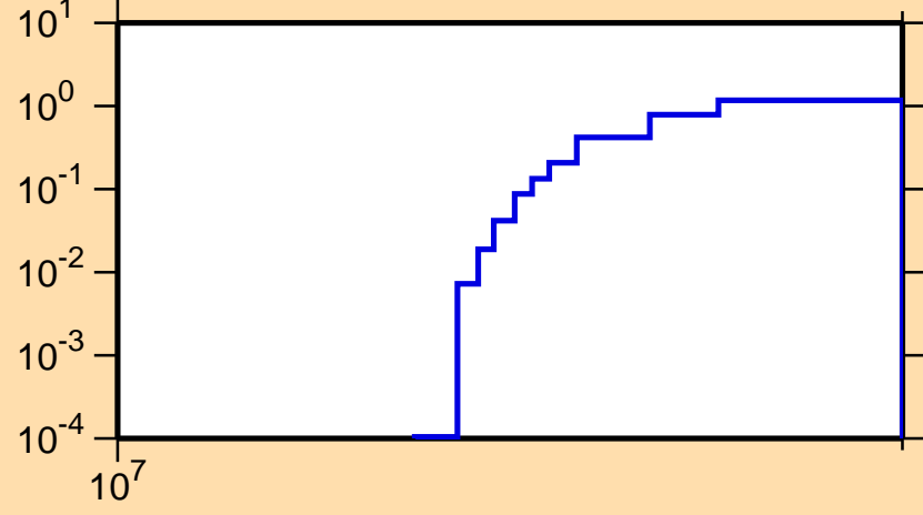
\sigma vs. E for ^{202}\text{Au}(n,3n)
