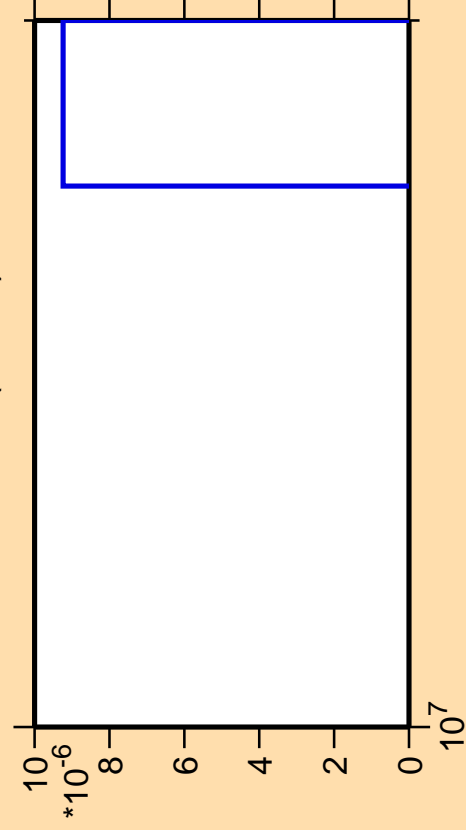
\Delta\sigma/\sigma vs. E for ^{202}\text{Au}(\text{mt } 11)
