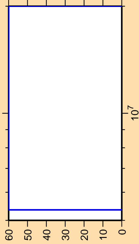
\Delta\sigma/\sigma vs. E for ^{202}\text{Au}(n,p)
