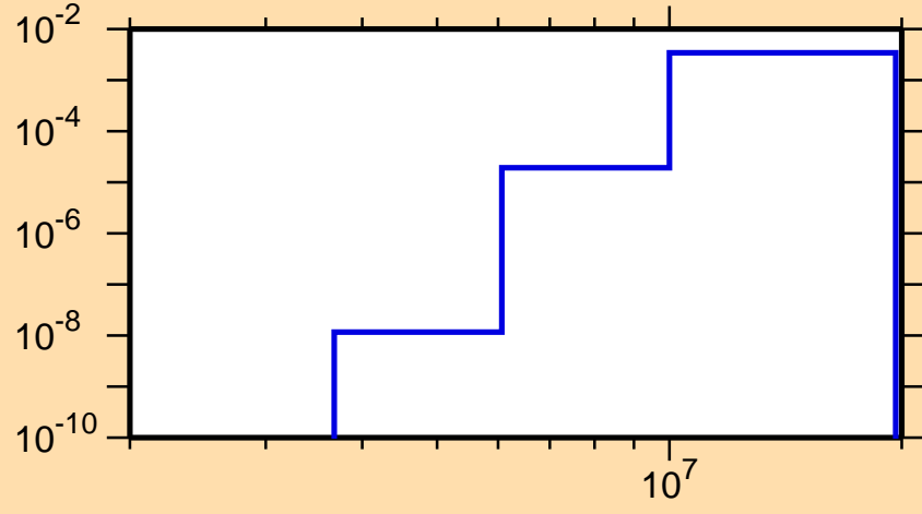
\sigma vs. E for ^{202}\text{Au}(n,p)
