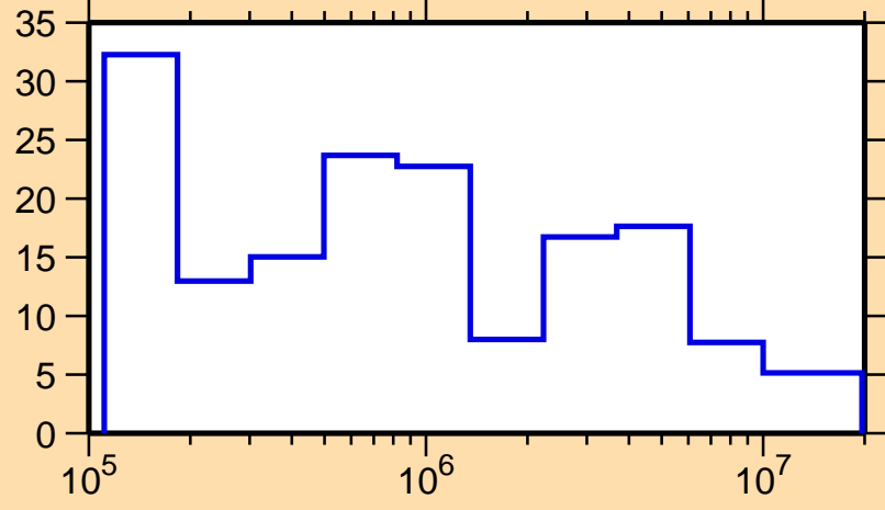
\Delta\sigma/\sigma vs. E for ^{202}\text{Au}(n,tot.)
