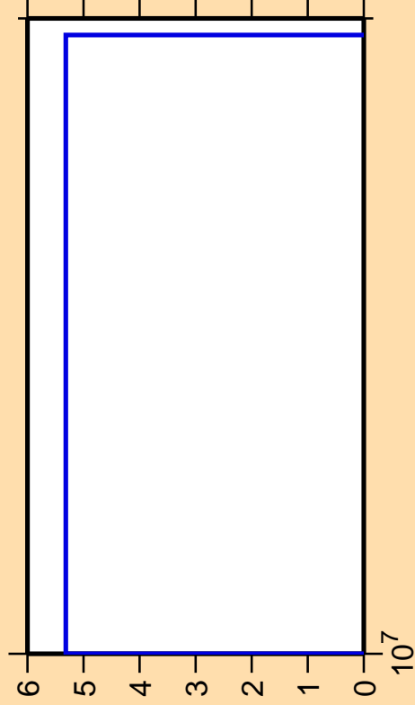
\Delta\sigma/\sigma vs. E for ^{202}\text{Au}(n,2n\alpha)
