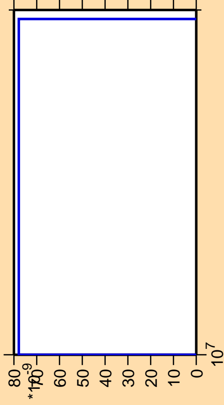
\Delta\sigma/\sigma vs. E for ^{202}\text{Au}(\text{mt } 11)
