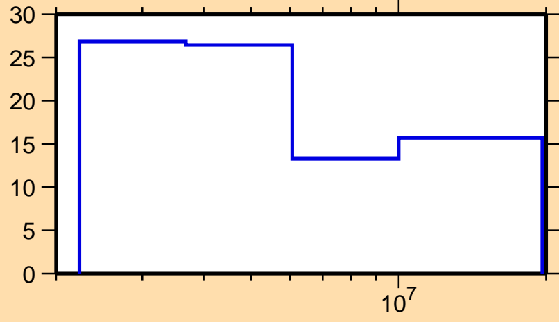
\Delta\sigma/\sigma vs. E for ^{202}\text{Au}(n,el.)
