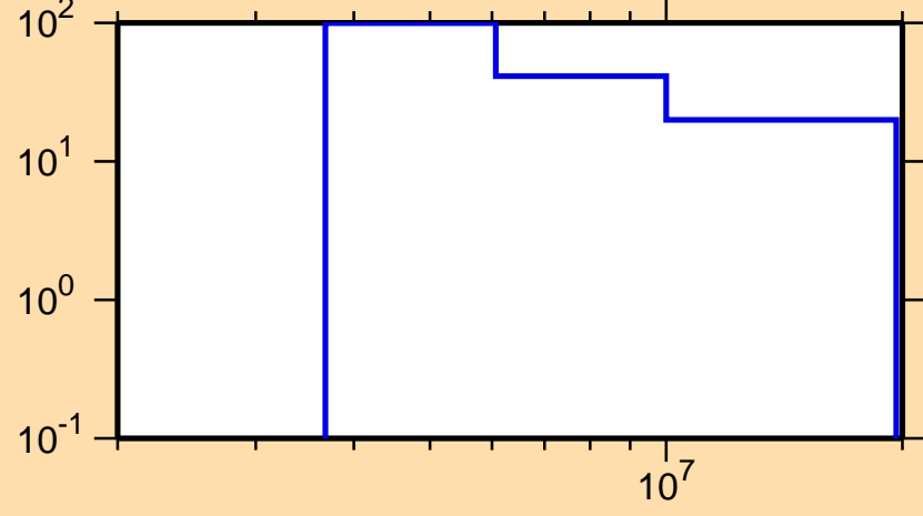
\Delta\sigma/\sigma vs. E for ^{202}\text{Au}(n,2n)
