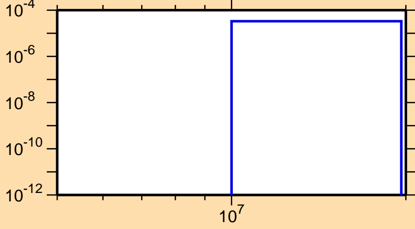
\sigma vs. E for ^{202}\text{Au}(n,d)
