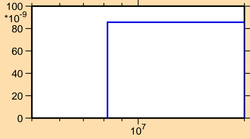
\sigma vs. E for ^{202}\text{Au}(n,n\alpha)
