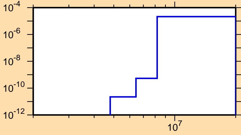
\sigma vs. E for ^{202}\text{Au}(n,\alpha)
