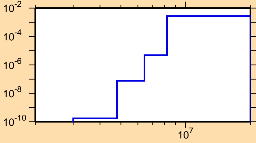
\sigma vs. E for ^{202}\text{Au}(n,p)
